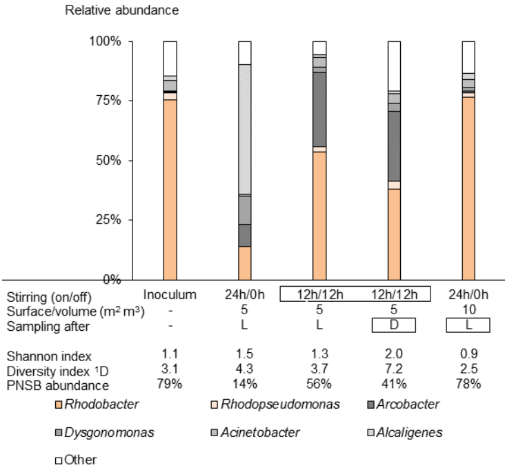
Figure 5 Effect of operational strategy of a raceway reactor on microbial community composition, Shannon's H' index, exp(H') and purple non-sulfur bacteria (PNSB) abundance. Raceway reactor operated at a sludge retention time of 2 d, testing the effect of oxygen (stirring) and the combination of light (surface-to-volume ratio). Sampling occurred after the light (L) or dark (D) period. Stirring (on/off) 12 h / 12 h implies stirring during the light period and not during the dark. The PNSB genera Rhodobacter and Rhodopseudomonas are marked in orange. Rectangular boxes show the change in reactor operation relative to the benchmark.
