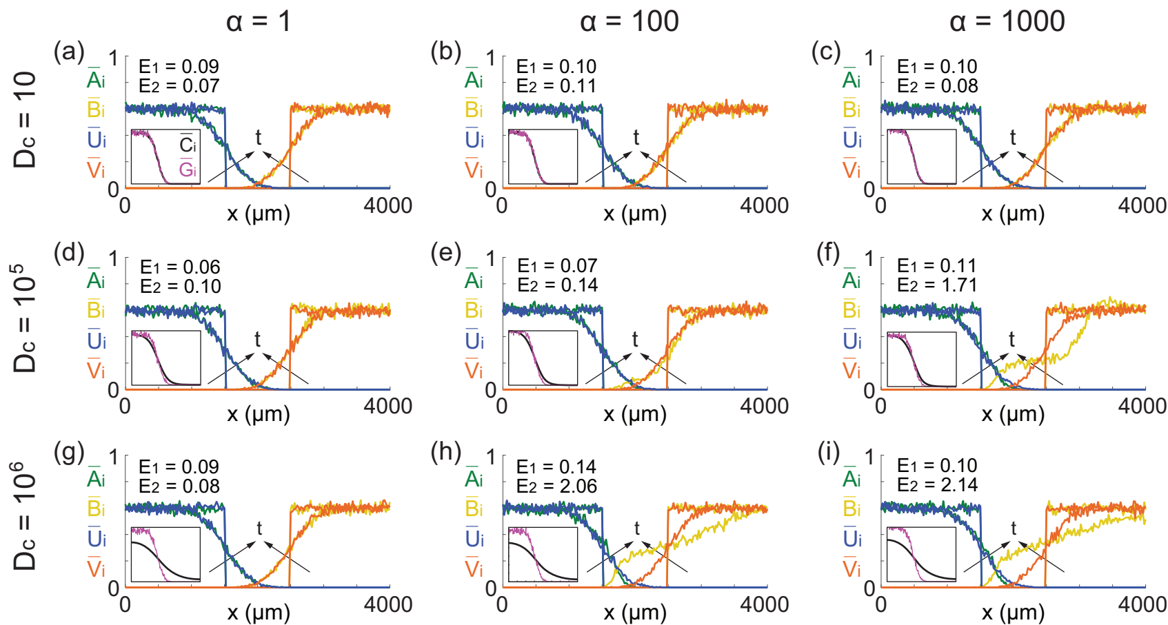
Fig. 6. Comparisons of the results from the full and reduced discrete models. Density profiles of Subpopulation 1 and Subpopulation 2 from the full and reduced discrete models at t = 0 and 24 h are shown. The inset in each subfigure compares \bar{C}_i and \bar{G}_i at t = 24 h. The black arrow indicates increasing time. D_a = D_b(0) = D_u = D_v(0) = 2000 \mu\text{m}^2/\text{h} , \lambda = 1 \mu\text{M}/\text{h} , \kappa = \mu = 1 / \text{h} , \Delta = 20 \mu\text{m} and \tau = 0.01 h for all the simulations.
