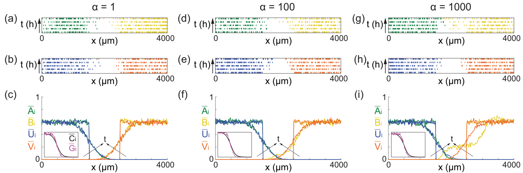
Fig. 4. Comparison of the full and reduced discrete models. (a), (d), (g) Snapshots from the full discrete model at t = 0, 6, 12, 18 , and 24 h. The arrow along the vertical direction indicates increasing time. (b), (e), (h) Snapshots from the reduced discrete model at t = 0, 6, 12, 18 , and 24 h. (c), (f), (i) Density profiles of Subpopulation 1 and Subpopulation 2 from the full and reduced discrete models at t = 0 and 24 h. The black arrow indicates increasing time. The inset in each subfigure shows profiles of the \bar{C}_i and \bar{G}_i at t = 24 h. All the simulation data are obtained by averaging over 500 statistically identically prepared realisations. D_a = D_b(0) = D_u = D_v(0) = 2000 \mu\text{m}^2/\text{h} , D_c = 10^5 \mu\text{m}^2/\text{h} , \lambda = 1 \mu\text{M}/\text{h} , and \kappa = \mu = 1/\text{h} , \Delta = 20 \mu\text{m} and \tau = 0.01 h for all the simulations.
