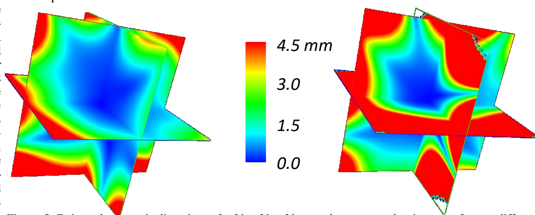
Figure 5: Estimated geometric distortions of a 30 x 30 x 30 cm volume centered at isocenter for two different ONDRI centers. Each scanner has a unique distortion characteristic when estimated using the LEGO® phantom.
