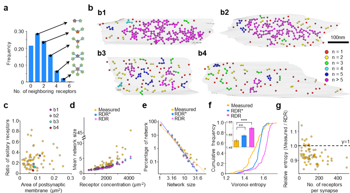
Fig. 3 | Two dimensional networks of GABA A Rs. a , Distribution of the number receptors with different numbers of 11-nm neighbors. b , Four examples ( b1-4 ) of receptor network organization on the postsynaptic membrane. Color indicates network size ( n , the number of receptor in a network). c , Scattered plot of the ratio of solitary receptors vs. the area of postsynaptic membrane for each synapse. Colored dots (magenta, gray, cyan and red) correspond to synapses in ( b ). d , Scattered plot of mean network size vs. receptor concentration for measured receptors (Measured), randomly distributed receptors (RDR), and randomly distributed receptors without overlap (RDR*). e , Power law distribution of network size in log-log plot. f , Cumulative frequency of Voronoi entropy for each synapse ( n=70 ). Inset: Mean value of Voronoi entropy. **, P<0.01 , ***, P<0.001 , K-S test. g , Scattered plot of relative entropy (defined as Measured/RDR) vs the number of receptors for each synapse.
