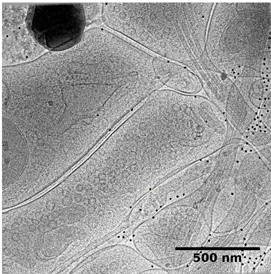
Supplementary Video 1 | Tilt series of an inhibitory synapse. This video shows the tilt series of an inhibitory synapse (same data as in Fig. 1b) obtained using VPP, electron filter and counting technologies. Black dots of 15-nm diameter are gold beads used as fiducial markers for image alignment.
