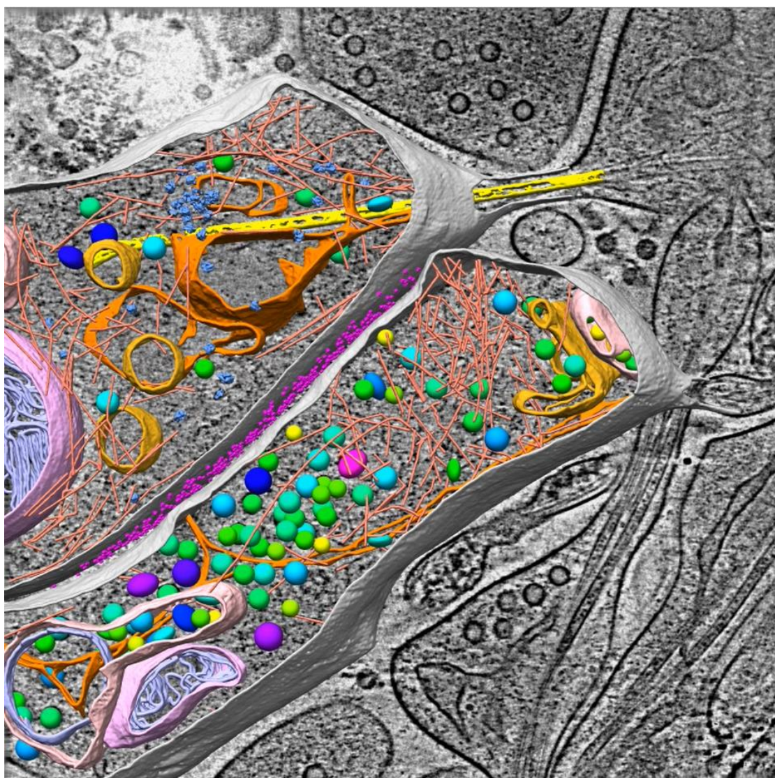
Supplementary Video 2 | Structures of an inhibitory synapse. This video shows the tomogram of the same synapse as in Fig. 2b, displayed as z-stack and 3D surface rendering of the segmented structures. The structures were colored same as Fig. 1c and Fig. 1d.
