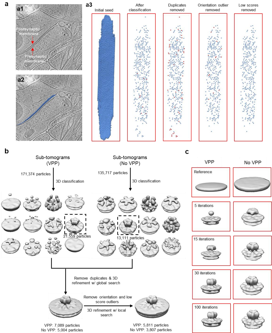
Extended Data Fig. 1 | Flowchart illustrates identification and sub-tomogram averaging of GABA A R. a , Steps for identifying GABA A Rs from sampling points. a1 , Electron tomographic slice of an inhibitory synapse. a2 , Electron tomographic slice superposed with sampling points on postsynaptic membrane. a3 , Sampling points after each step. Red points are sampling points that will be discarded in the next step. b , Classification
