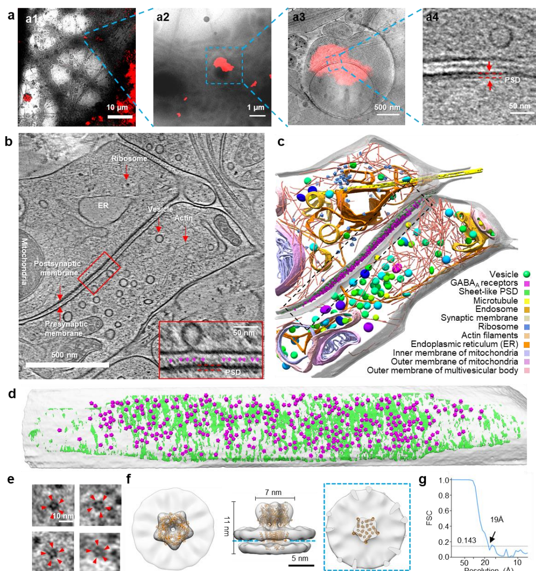
Fig. 1 | Identification and in situ structure of GABA A R in inhibitory synapse. a , Identification of inhibitory synapses with cryo-correlative light and electron microscopy. a1 , Low magnification EM image superposed with fluorescence image of gephyrin-mCherry. a2 , Zoomed-in view of ( a1 ). a3 , Electron tomographic slice superposed with fluorescence puncta. a4 , Zoomed-in view of ( a3 ) showing thin sheet-like PSD. b , A tomographic slice of an inhibitory synapse. Various subcellular components are labelled on the image. Inset: Zoomed-in view showing receptor densities (magenta arrowheads). c , 3D rendering of the tomogram shown in ( b ). d , Front view of GABA A Rs (purple), density of the scaffolding protein layer (green) on the postsynaptic membrane (transparent gray). e , Example tomographic slices of individual GABA A R in top view. Red arrowheads showing 5 blobs of
