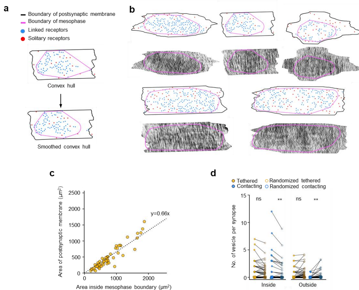
Extended Data Fig. 7 | Mesophasic assembly of PSD. a , Example of convex hull and smooth convex hull of linked receptors. b , Examples of receptors distributions and 2D density profiles of scaffolding layer. c , Scatted plot of area inside mesophase boundary and area of postsynaptic membrane, fitted with a dashed line. d , Comparison between the number of either type of vesicles inside or outside of mesophase boundary with the corresponding number based on randomized vesicle distribution within the whole synapse (n=58 synapses). ns, P=0.20; **, P=0.005, paired two-tailed t-test.
