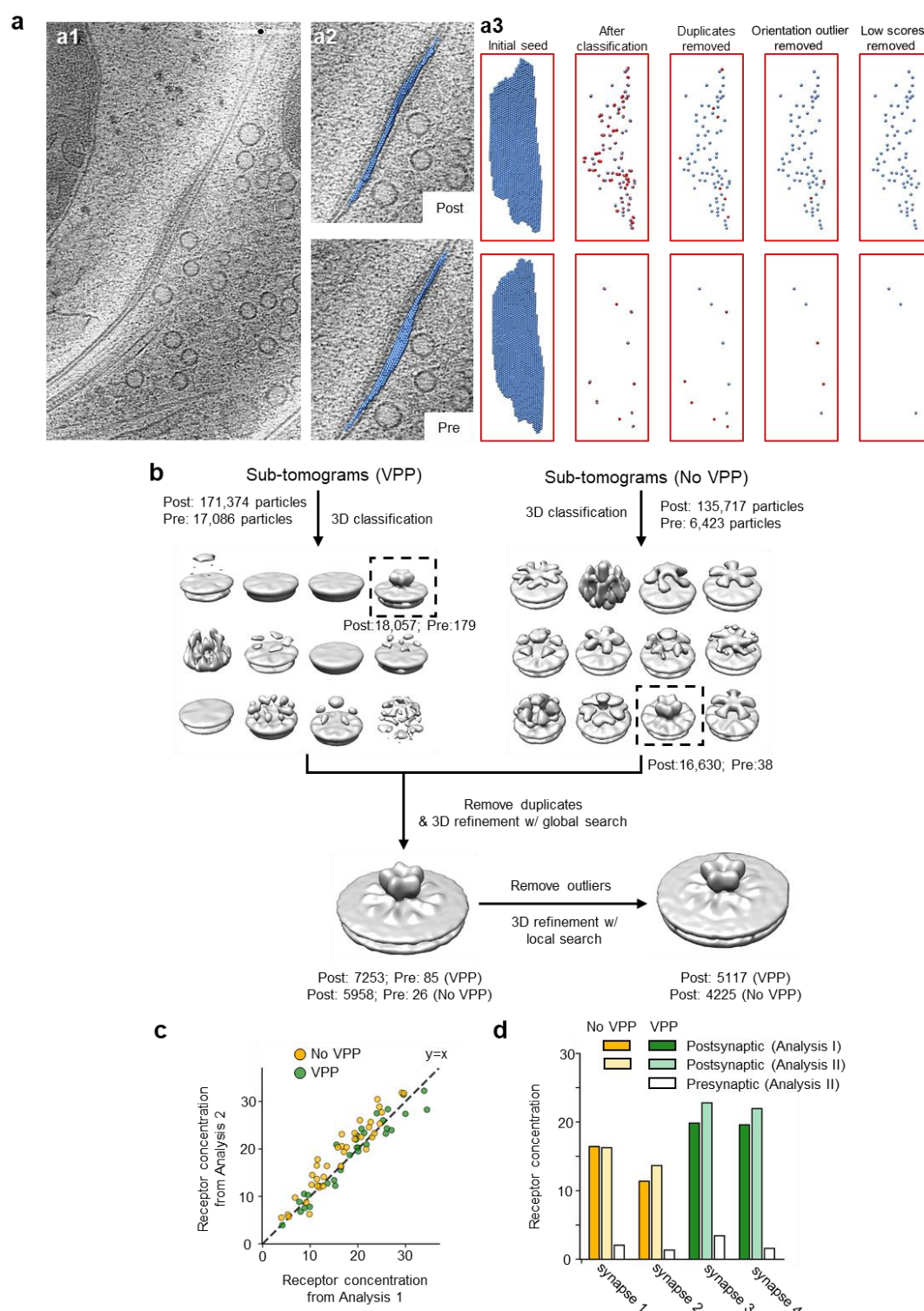
Extended Data Fig. 3 | Identification of GABA A Rs using sub-tomograms mixed with sub-tomograms on presynaptic membrane. a , Steps for identifying GABA A Rs from sampling points mixed with sub-tomograms on presynaptic membrane. a1 , Electron tomographic slice of an inhibitory synapse. a2 , Electron tomographic slices superposed with sampling points on postsynaptic membrane (top) or presynaptic membrane (bottom). a3 ,
