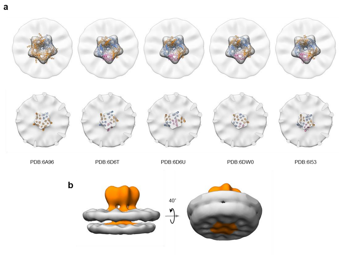
Extended Data Fig. 5 | Structure features of sub-tomogram average of GABA A R. a, Density of the sub-tomogram average fitted with atomic models of different subunit compositions or conformations 26-29 . b, Left: Sub-tomogram average of GABA A R. Orange density is GABA A R density. Gray density is membrane bilayer. Right: Rotated view of sub-tomogram average of GABA A R displayed at low threshold.
