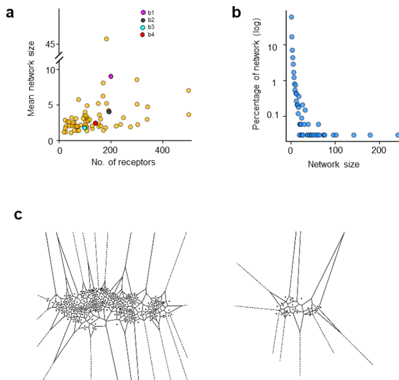
Extended Data Fig. 6 | Two dimensional networks of GABA A Rs. a , Scattered plot of mean network size (number of receptors divided by number of networks) and number of receptors for each synapse. Colored dots (magenta, gray, cyan and red) correspond to the four synapses in Fig. 3b respectively. b , Distribution of network size. Y-axis is plot in logarithm scale. c , Examples of Voronoi tessellation of receptors on postsynaptic membrane. Black dots represent the localizations of GABA A Rs.
