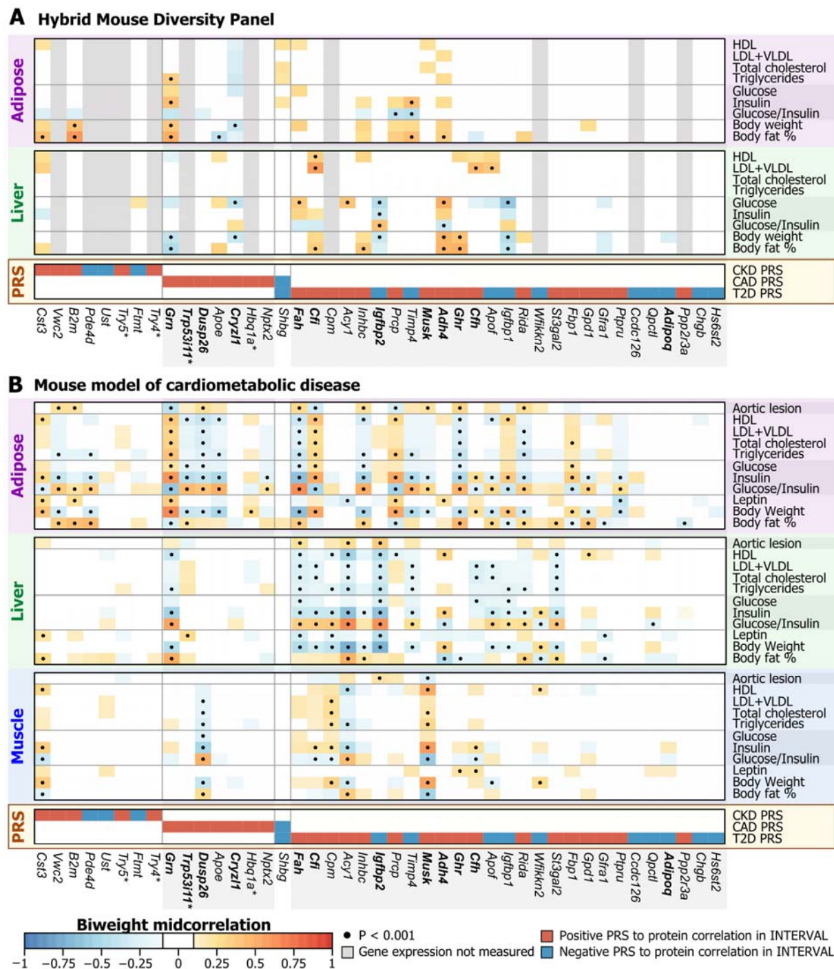
Figure 4: Tissue-specific gene expression and cardiometabolic traits in mice
