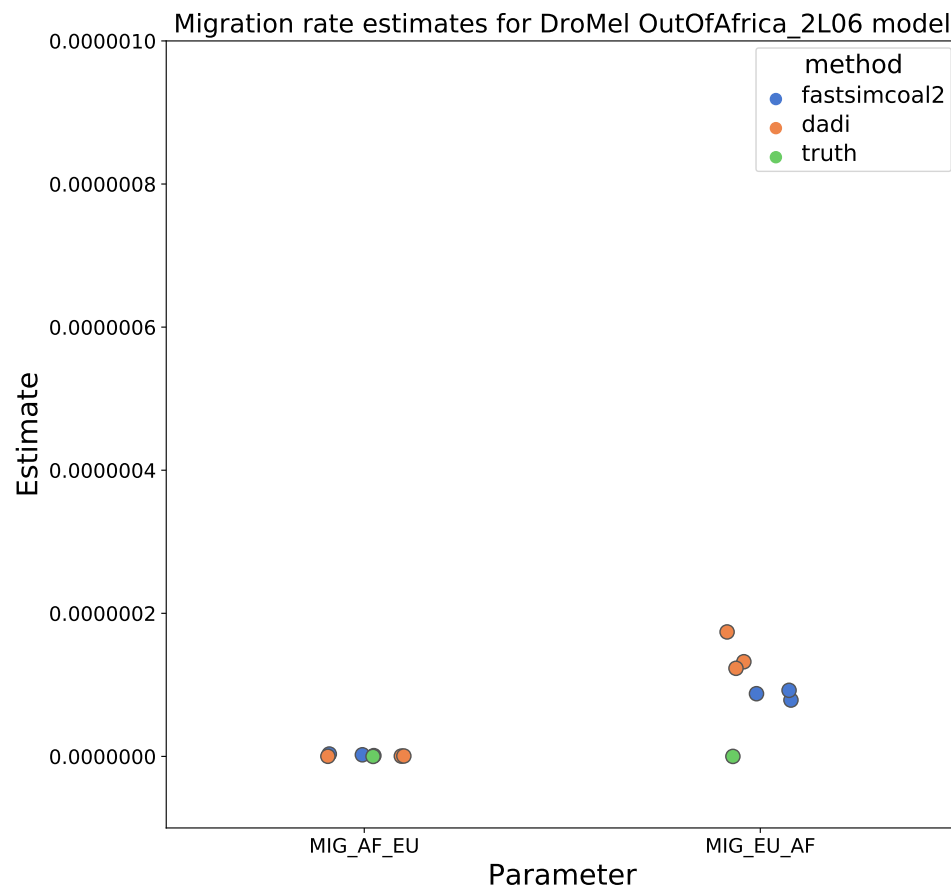
Figure S6: Migration rate parameters estimated under a two-population Drosophila model. Here we show inferred migration rates from ∂a∂i and fastsimcoal2 . Data were generated by simulating replicate Drosophila genomes under the Li and Stephan (2006) model and using the genetic map inferred in Comeron et al. (2012).
