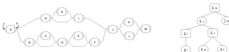
Fig. 1. Example sequence graph (left) and its snarl tree (right). Chains in the sequence graph are represented as rectangular nodes in the snarl tree and snarls are represented as elliptical nodes.
