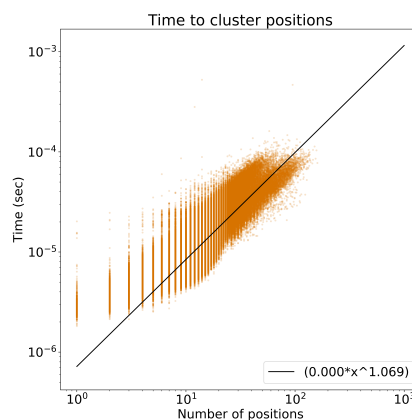
Fig. 9. Run time growth of our clustering algorithm. The regression line suggests that the run time of our algorithm is nearly linear in the number of positions.
