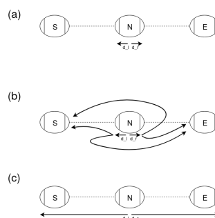
Fig. 5. (a) S and E are the boundary nodes of a structure that contains a child structure N . d_l and d_r are the minimum distances from some object in N to the ends of N . (b) The minimum distances from each end of N to \bar{s} and e are found using the minimum distance index. (c) By adding the appropriate distances and taking the minimums, we can get the minimum distances to s and \bar{e} .
