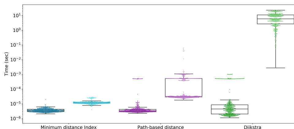
Fig. 7. Run times for distance algorithms. Random pairs of positions were chosen from either within a read-length random walk (dark colors) or randomly from the graph (light colors).
