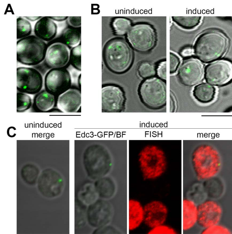
Figure 5. Expression of the model RNA does not induce formation of P bodies. (A): Live-cell imaging of non-transformed EDC3-GFP strain. Generally, under normal conditions, between 1 and 3 small P bodies per cell are detected. (B and C): The model RNA was expressed in EDC3-GFP strain as in Figure 2. Uninduced cells were used to control for P bodies unrelated to the expression of the model RNA and for unspecific FISH signal. (B): Live-cell imaging of EDC3-GFP strain. Expression of the model RNA leads to the increase in neither the size nor the number of P bodies per cell. (C): FISH-IF of the model RNA and Edc3-GFP showed that the granules of the model RNA are distinct from P bodies, although some of them may be located in the vicinity of each other. In (A) and (B), overlay of Edc3-GFP signal and bright field is shown. In (C), "FISH" corresponds to FISH detection of the model RNA, "Edc3-GFP/BF" corresponds to overlay of bright field and Edc3-GFP signal and "merge" corresponds to overlay of bright field, FISH and Edc3-GFP labeling. Scale bar is 5 \mu m.
