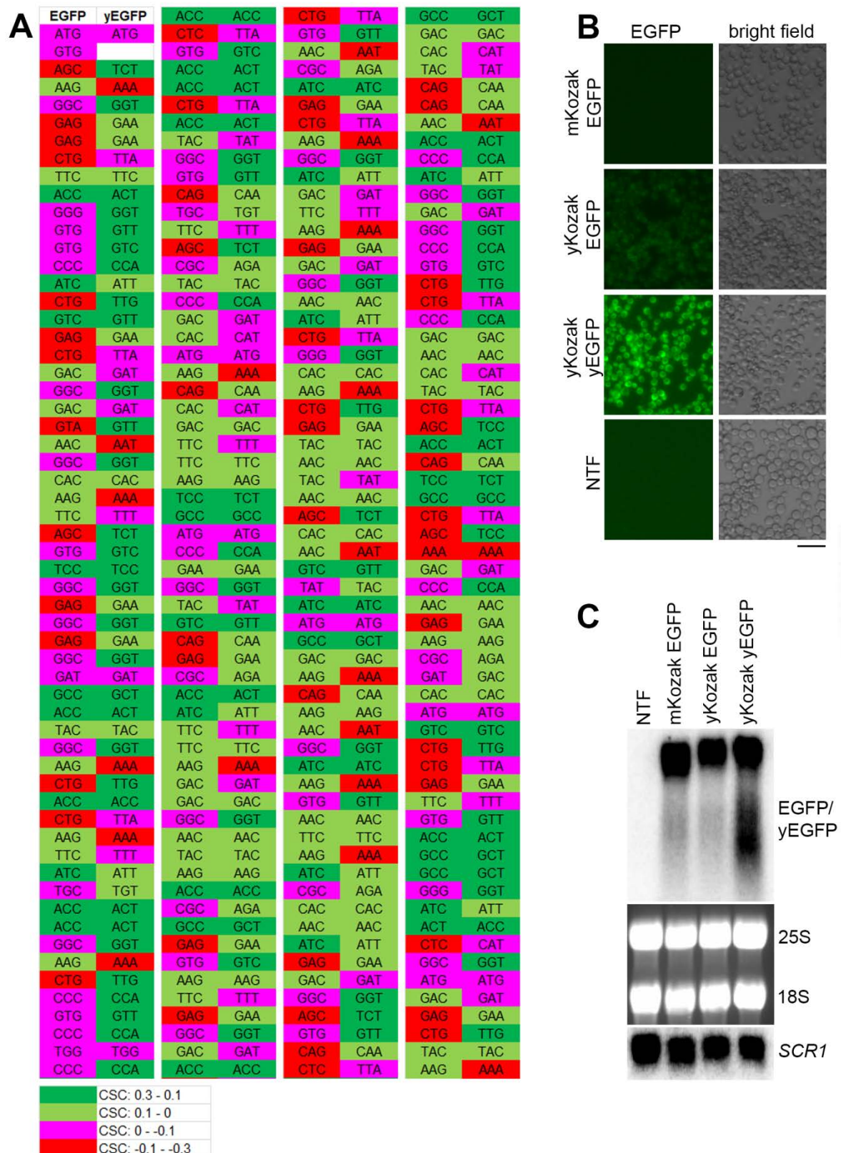
Figure 1. The steady state level of the model RNA is unaffected by its suboptimal codon bias. (A): comparison of codon optimality for expression in yeast between EGFP and yEGFP . CSC was attributed to each amino acid codon according to [22] and color-coding was added, as indicated in the lower panel. For image convenience the open reading frame (ORF) of EGFP and yEGFP was divided in four regions depicted from left to right and separated by vertical white line. (B): EGFP
