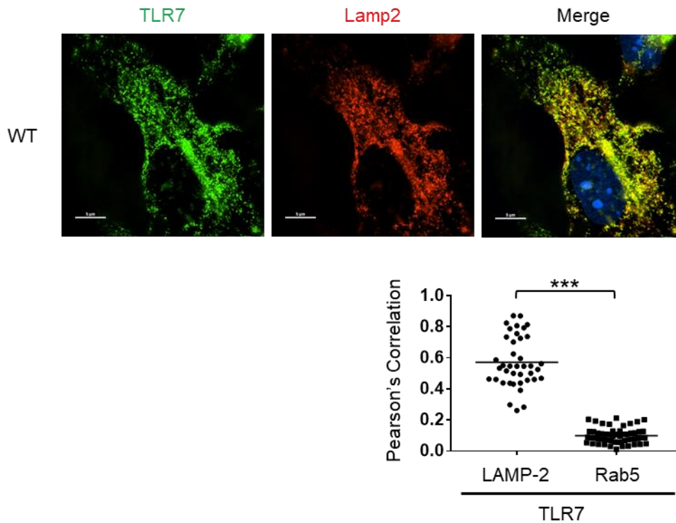
Figure S11. TLR7 is localized to LAMP-2-positive vesicles
