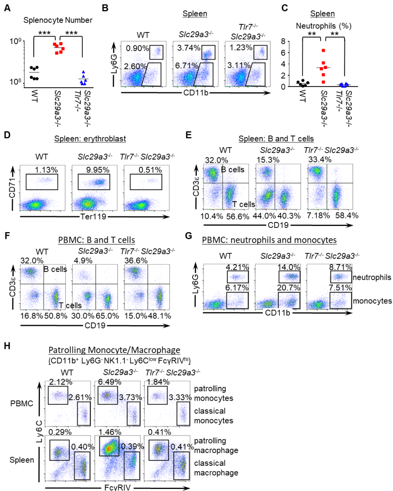
Figure S4. TLR7-dependent monocytosis in Slc29a3 -/- mice
