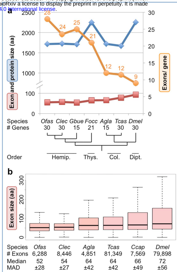
Fig 6. Trends in gene structure show hemipteroid-specific tendencies.
