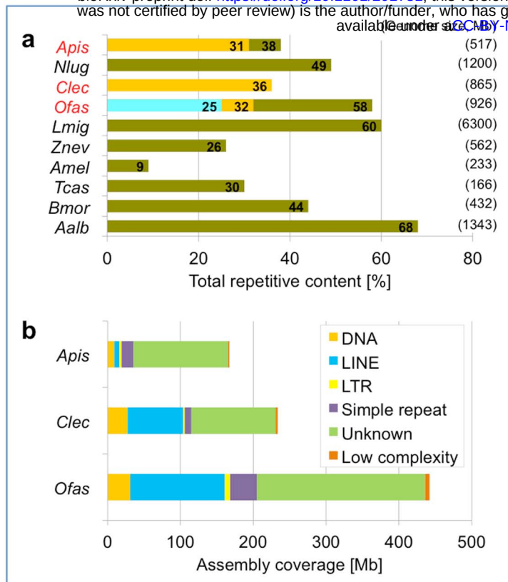
Fig 5. Comparison of repeat content estimations.
