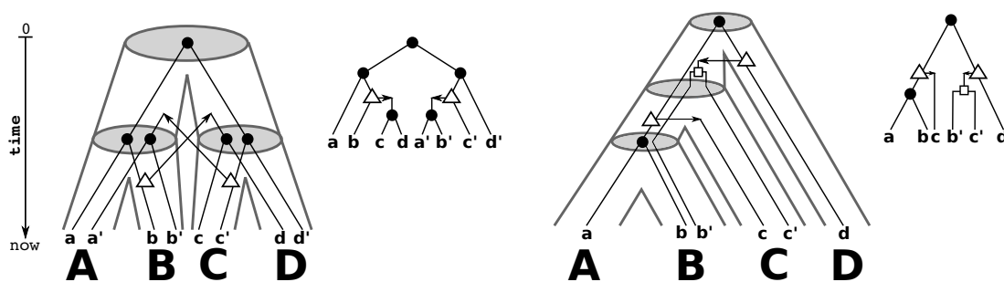
Figure 2: Shown are two (tube-like) species trees with reconciled gene trees. The reconciliation map \mu for T and S is given implicitly by drawing the gene tree (upper right to the respective species tree) within the species tree. In the left example, the map \mu is unique. However, \mu is not time-consistent and thus, there is no time consistent reconciliation for T and S . In the example on the right hand side, \mu is time-consistent.
