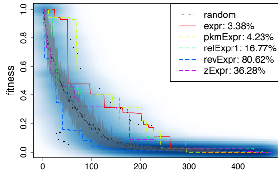
Fig. 3. Fitness decrease while removing genes from the iMK735 model with different rankings in the UH condition (UH2 sample). random: random draw, expr: voom-normalized expression, pkmExpr: voom-normalized expression in RPKM, relExpr1: relative expression \text{expr}/\langle \text{expr} \rangle , revExpr: reverse expression, zExpr: z-score. Blue darkness in the scatter plot represents the density of random fitness. Gray region represents 20%-80% quantiles of random fitness.
