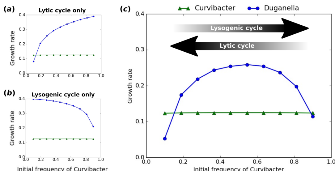
Figure 4 Growth rates obtained from the model during the exponential growth phase of Curvibacter sp. and Duganella sp. for different initial frequencies of Curvibacter sp. The two panels on the left show the growth rates if only the lytic (a) or lysogenic (b) phage life cycle is taken into account, respectively. (c) Bacterial growth rates if both life cycles are taken into account. The arrows indicate at which ends of the initial frequency spectrum the two different phage life cycles are most effective. Parameter values for this example: N_0 = 100 , B_0 = 10^5 , P_0 = 3.5 \times 10^4 , c = 10^{-5} , r_C = 0.125 , r_D = 0.4 , H = 0.05 , \phi = 10^{-8} , \beta = 50 , m = 0.25 , p = 0.05 .
