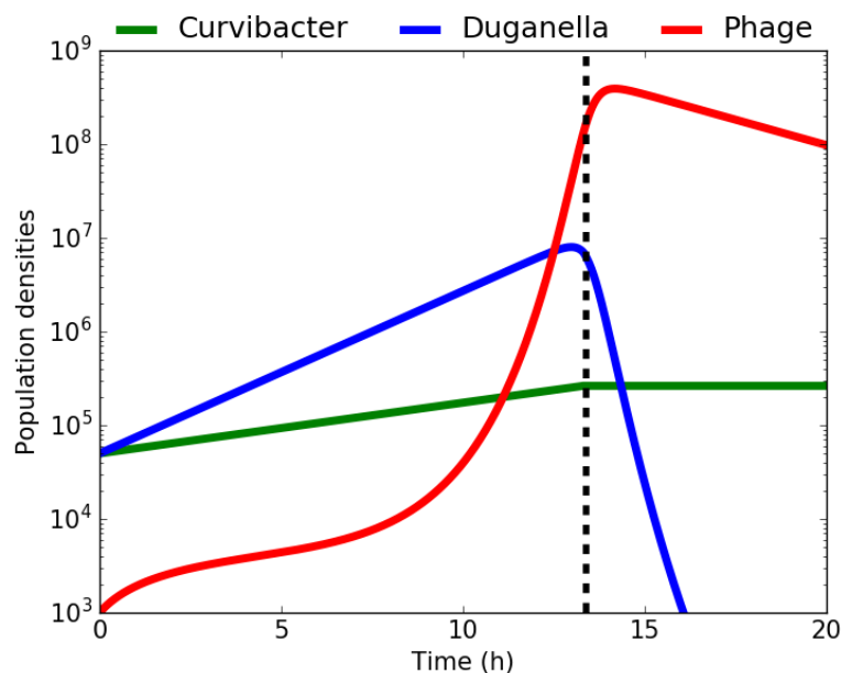
Suppl. Fig. 1 Typical population dynamics obtained from model (1). Both bacteria initially grow exponentially, until Duganella sp. growth declines due to lytic phage infections and Curvibacter sp. growth slows down due to depletion of nutrients, respectively. The vertical dashed line at t = t_{exp} indicates the end of the exponential growth phase, defined as the time when Curvibacter sp. growth ceases. Duganella sp. density approaches 0 after about 20 hours due to continued phage infections. Parameters values for this example: N_0 = 100 , B_0 = 10^5 , f_0 = 0.5 , P_0 = 10^3 , c = 10^{-5} , r_C = 0.125 , r_D = 0.4 , H = 0.05 , \phi = 10^{-8} , \beta = 50 , m = 0.25 , p = 0.05 .
