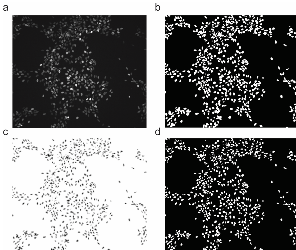
Supplementary Figure 2. Image processing steps for FUCCI-ReN nucleus images. (a) Fluorescence image from H2B-Cerulean channel marking all nuclei. (b) Binary mask obtained through adaptive thresholding. (c) Image obtained through imposing minimum of distance transform of binary image in (b) and local minima. This image serves as seeds for the watershed algorithm. (d) Final mask obtained after watershed transform.
