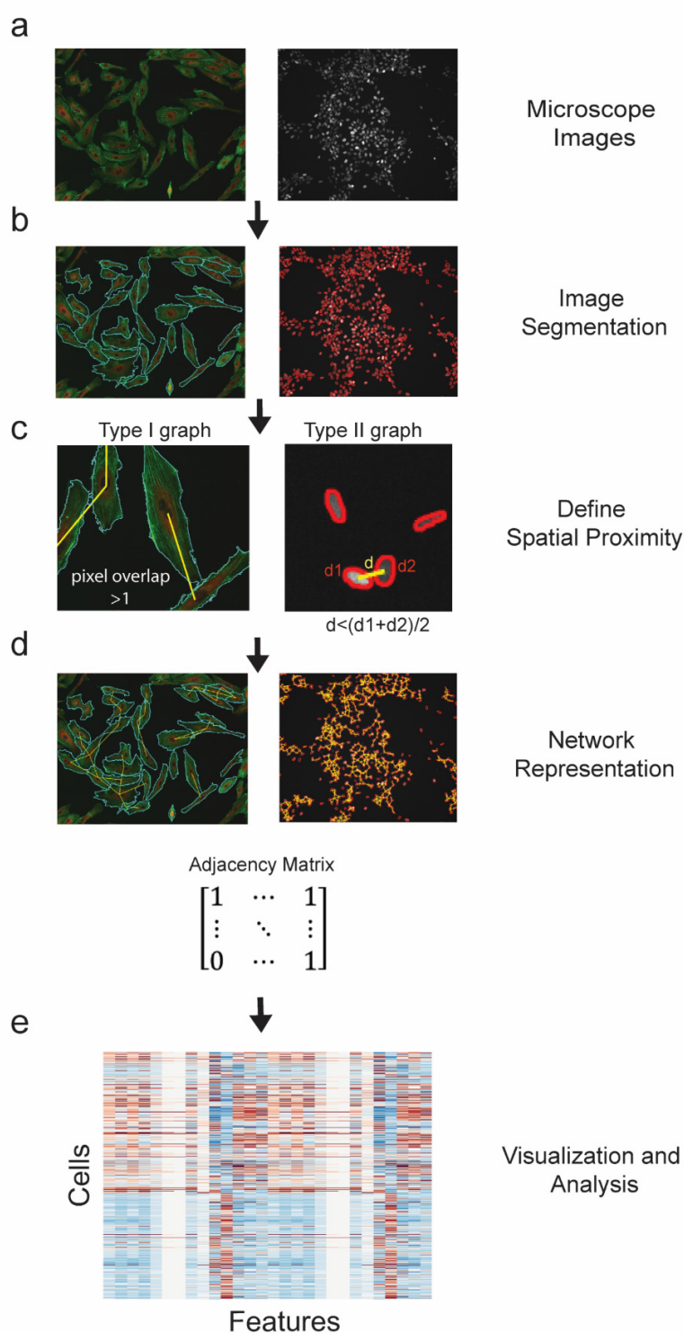
Figure 1. The cytoNet image-processing pipeline. (a) The pipeline begins with microscope images. (b) Segmentation algorithms automatically detect cell boundaries ( Supplementary Fig. 1, 2 ). (c) Spatial proximity is determined either by measuring shared pixels between cell pairs – type I graphs (left panel) or by comparing distance between cell centroids to a threshold distance – type II graphs (right panel). (d) We represent the resulting network as an adjacency matrix. (e) Metrics derived from the adjacency matrix are used to describe network information. These metrics are a list of features computed on a per-cell basis.
