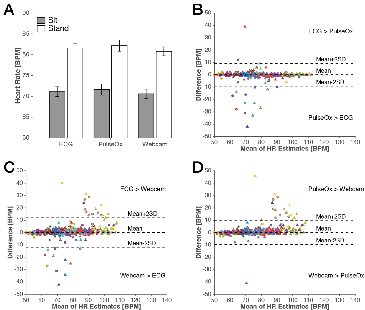
Figure 3. Results from the sitting vs. standing task. (A) Mean heart rate for sitting and standing from each measure. Error bars represent SEM, corrected for inter-individual differences (within-subject SEM; Loftus & Masson, 1999). Bland-Altman plots for pairs of measures: (B) ECG-PulseOx, (C) ECG-Webcam, and (D) PulseOx-Webcam. Markers represent each block of the task from each participant. Markers in distinct colors represent individual participants; measurements from sitting blocks are shown as circles, standing blocks are shown as triangles.
