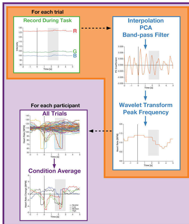
Figure 2. Demonstration of the analysis pipeline for an event-related design.
