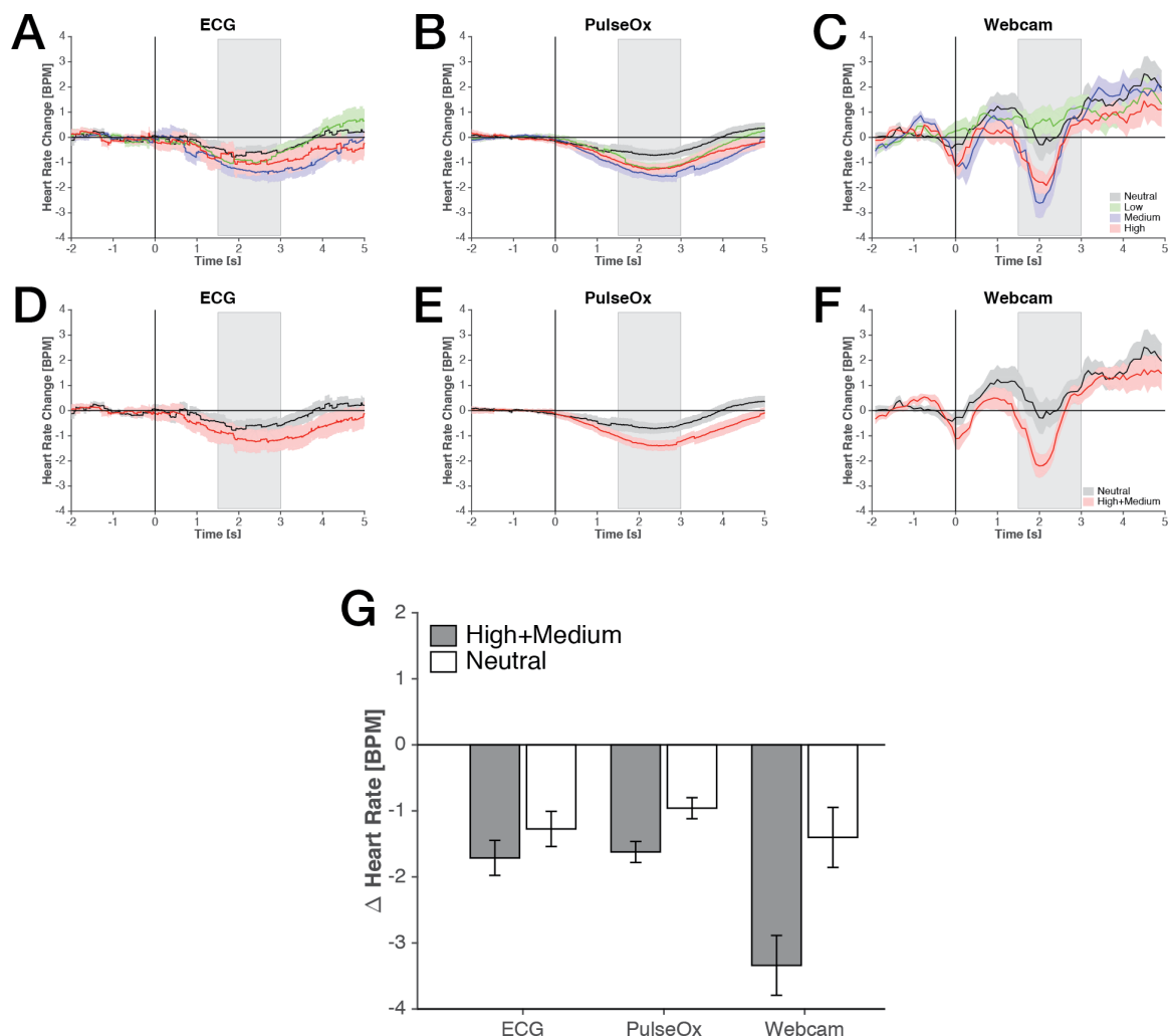
Figure 4. Results from the emotional and neutral picture-viewing task. Event-related changes in heart rate in response to viewing each of the picture types, as measured by the (A) ECG, (B) PulseOx, and (C) Webcam. Shaded error bars represent within-subject SEM. The shaded time window (1500-3000 ms) depicts the data used in the statistical analyses. (D-F) Re-plots panels A-C, collapsing the High and Medium arousal conditions and removing the Low arousal condition. (G) Mean heart rate deceleration related to stimulus presentation, relative to the pre-stimulus baseline. Error bars represent SEM, corrected for inter-individual differences (within-subject SEM; Loftus & Masson, 1999).
