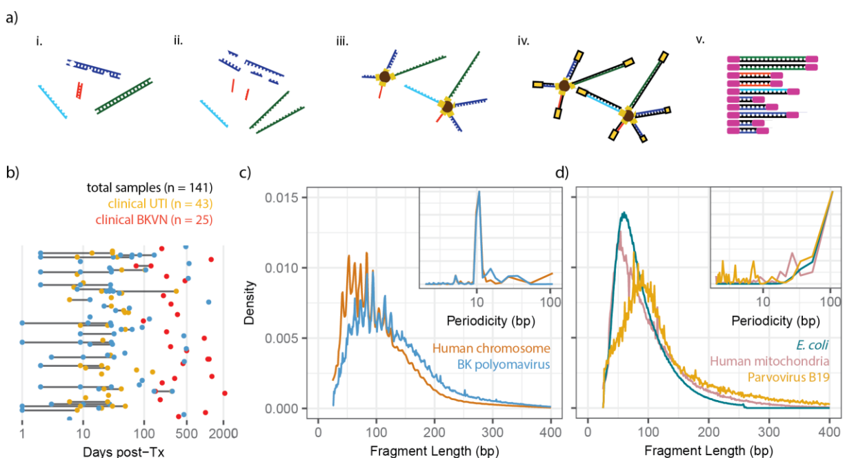
Figure 1. Shotgun sequencing assay and biophysical properties of urinary cfDNA.
