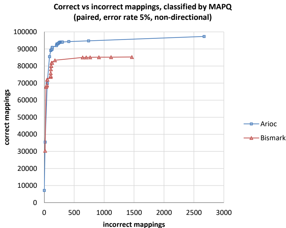
Figure 2. Total correctly mapped versus incorrectly mapped reads, plotted for decreasing MAPQ, for 100,000 simulated 100nt paired-end Illumina reads (200,000 mates).
