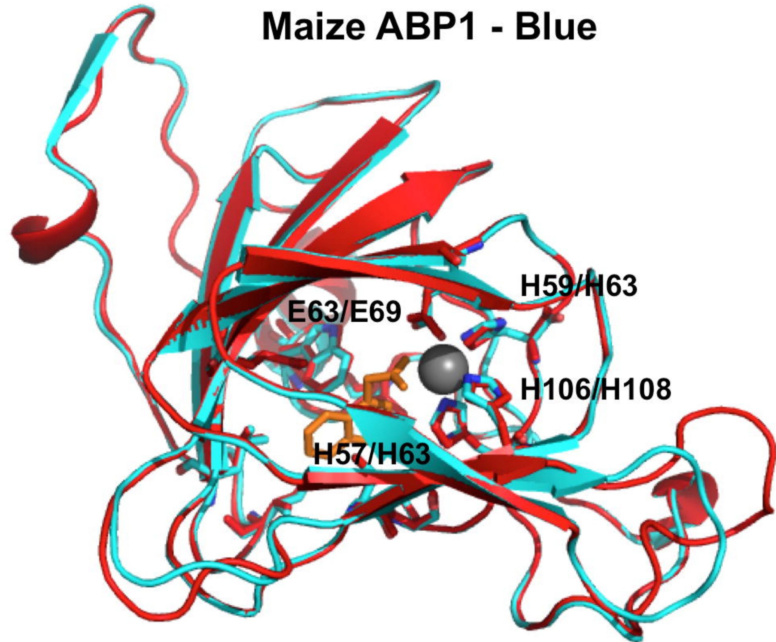
Zn 2+ chelation
