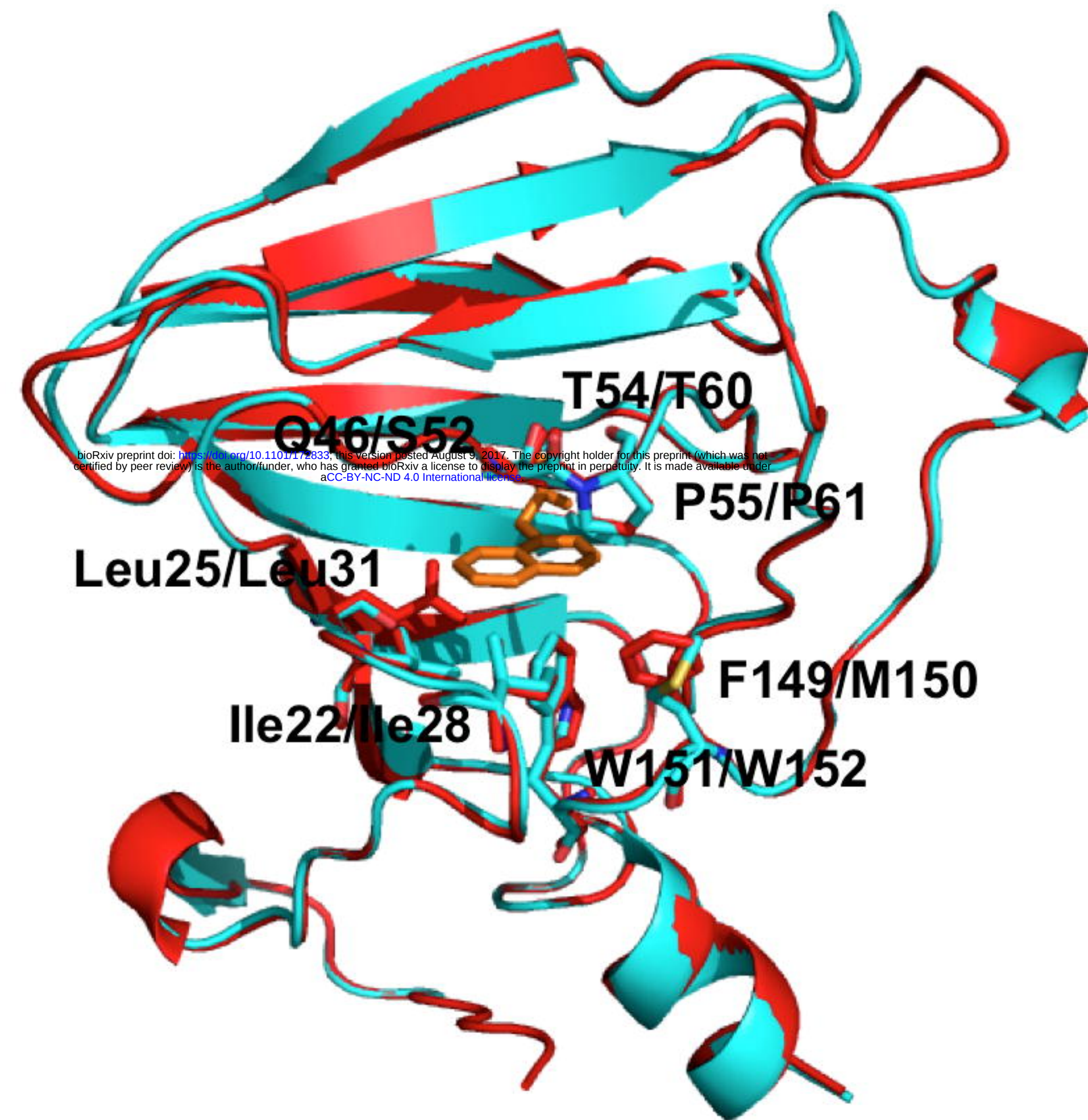
Hydrophobic pocket
