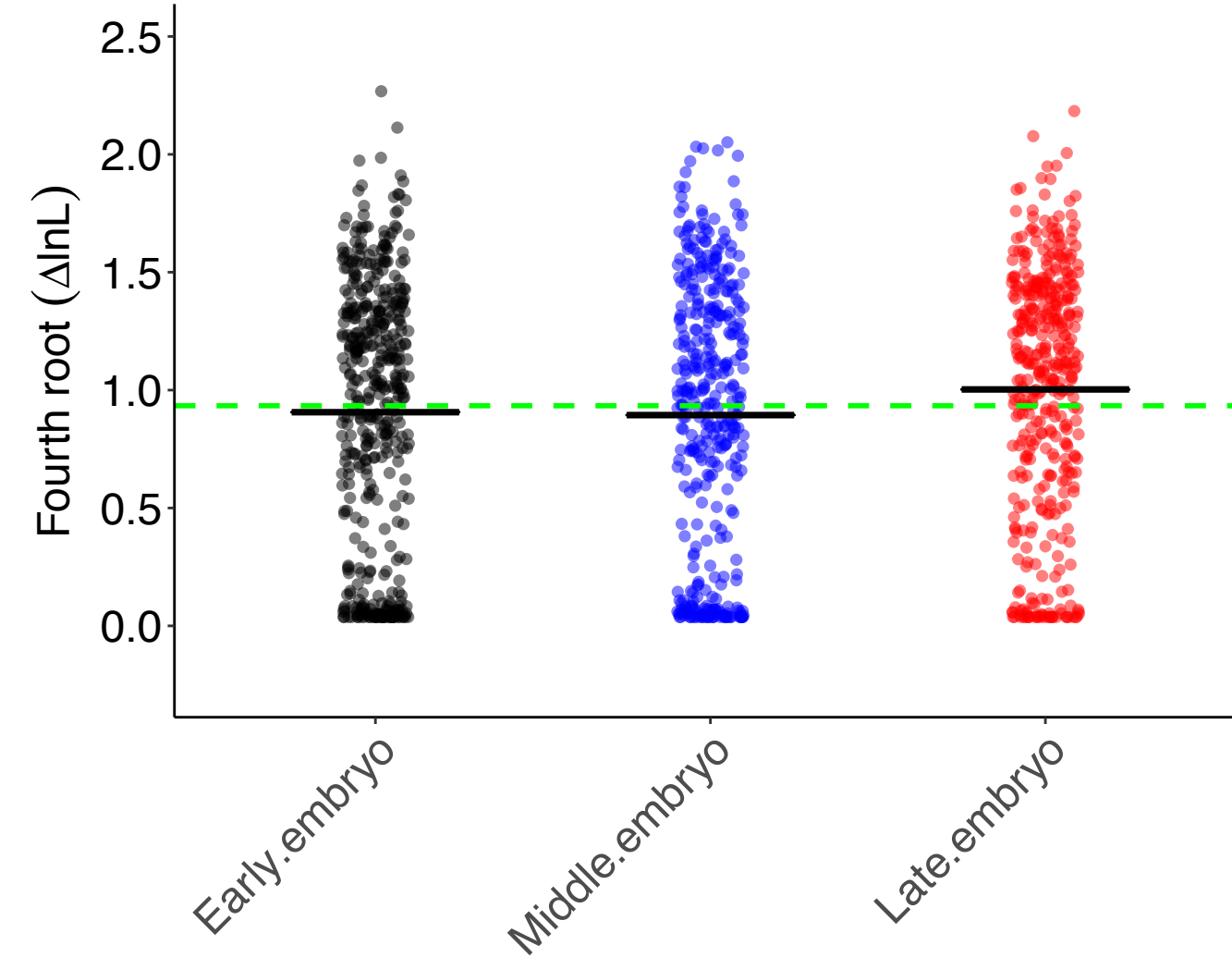
Murinae branch
