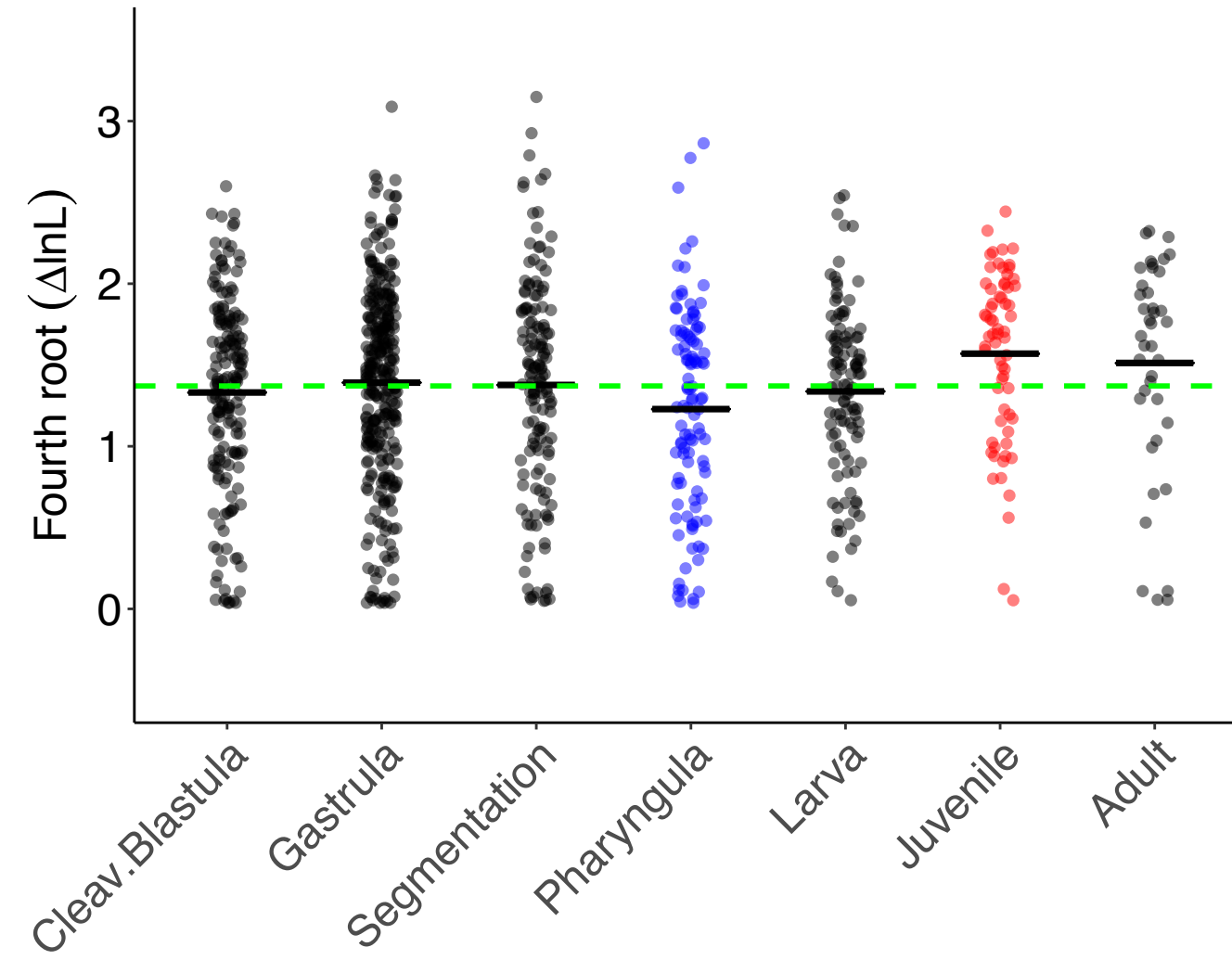
Clupeocephala branch
