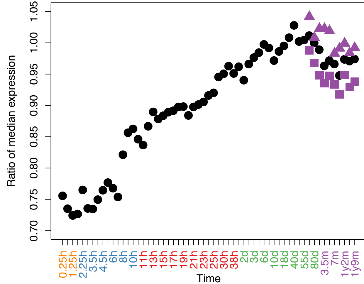
Clupeocephala branch
