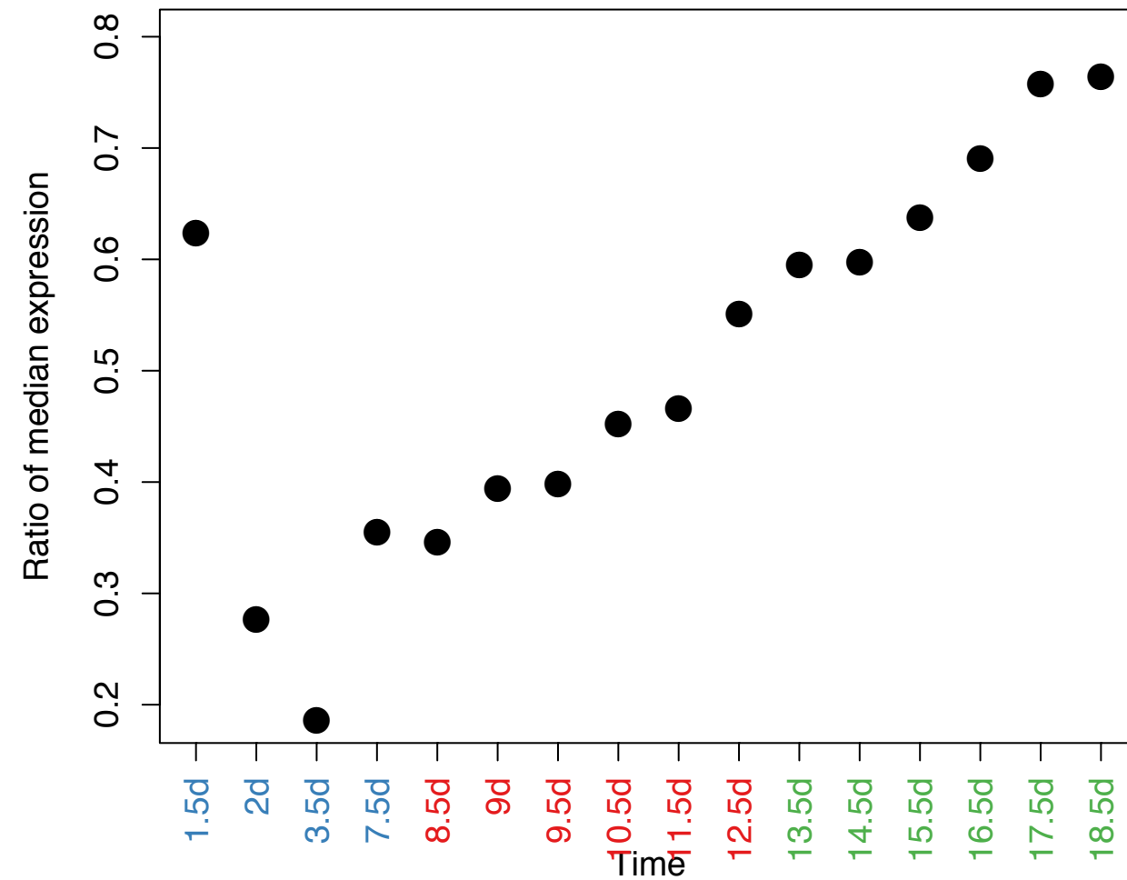
Murinae branch
