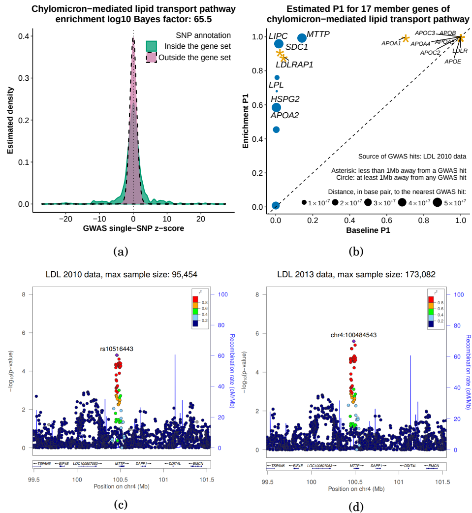
Fig 5: Enrichment of chylomicron-mediated lipid transport pathway in forms a strong association between a member gene MTTP and levels of low-density lipoprotein (LDL) cholesterol. (a) Distribution of GWAS single-SNP z-scores from summary data published in 2010 [35], stratified by gene set annotations. The solid green curve is estimated from z-scores of SNPs within \pm 100 kb of the transcribed region of genes in the chylomicron-mediated lipid transport pathway (“inside”), and the dashed reddish purple curve is estimated from z-scores of remaining SNPs (“outside”). This panel serves as a visual sanity check to confirm the observed enrichment. (b) Estimated posterior probability ( P_1 ) that there is at least one associated SNP within \pm 100 kb of the transcribed region of each pathway-member gene under the enrichment model ( M_1 ) versus estimated P_1 under the baseline model ( M_0 ). These gene-level P_1 estimates and corresponding SNP-level statistics are provided in Supplementary Table 4 . (c) Regional association plot for MTTP based on summary data published in 2010 [35]. (d) Regional association plot for MTTP based on summary data published in 2013 [58].
