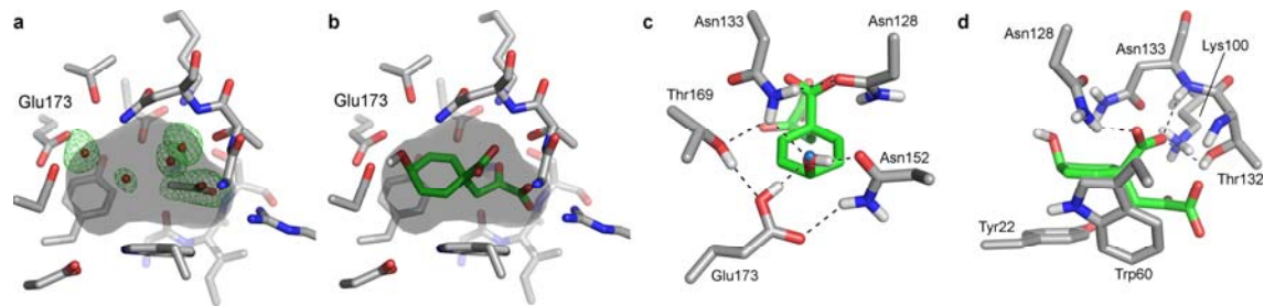
Figure 2. Crystal structure of PaCDT. a , Active site of PaCDT. The surface of the active site is shown in grey. Electron density for water and acetate molecules is shown by an omit mF_o - DF_c map contoured at +3\sigma . b , Structure of the PaCDT-prephenate complex predicted by computational docking. Docking with L-arogenate yielded a similar pose. c , Glu173 is poised for proton donation to the departing hydroxyl group of prephenate by hydrogen bonding interactions with neighboring residues. The position predicted to be occupied by the hydroxyl group of prephenate is occupied by a water molecule in the unliganded PaCDT structure (blue sphere). d , \pi -stacking interactions with Tyr22 and Trp60, and polar interactions with Lys100, Asn128, Thr132, and Asn133 could contribute to transition state stabilization.
