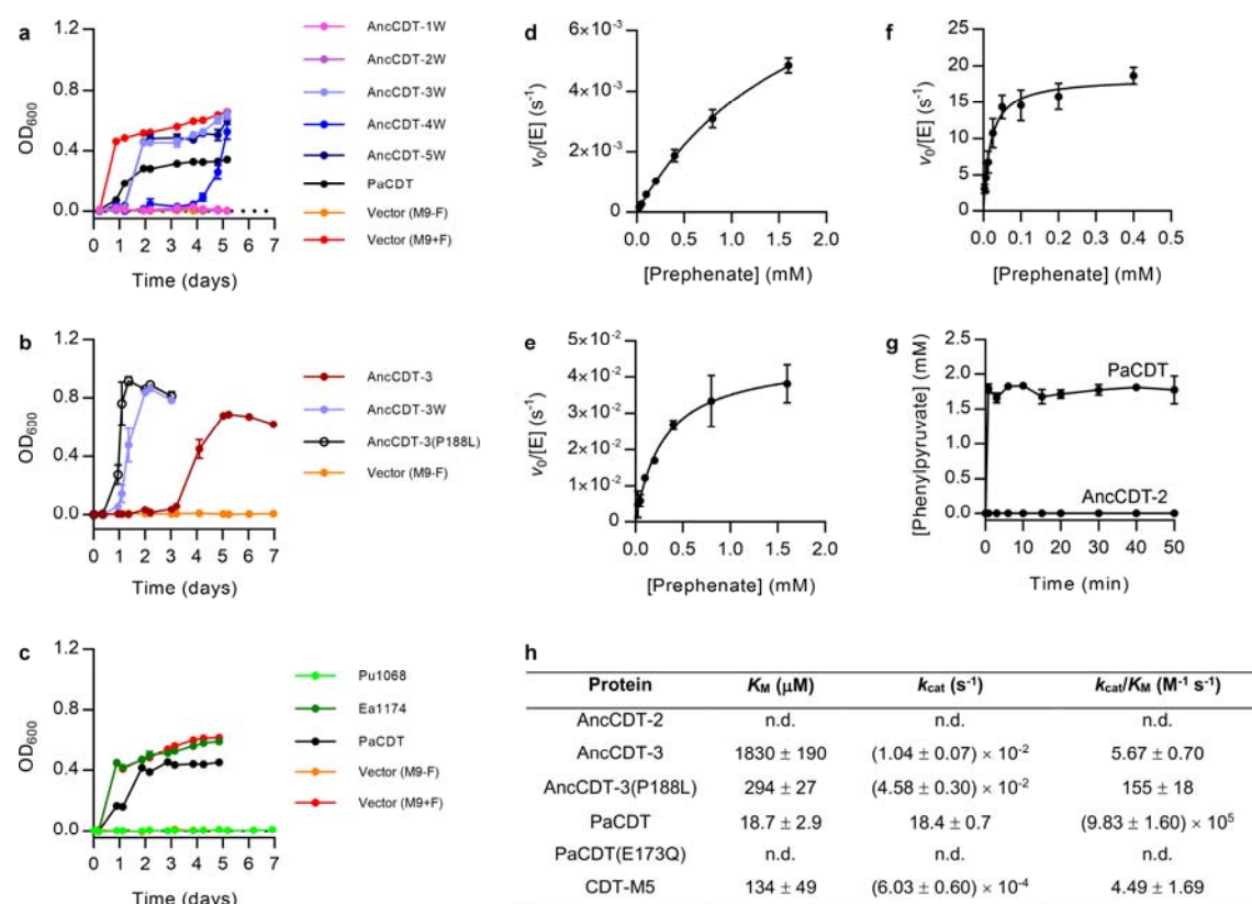
Extended Data Figure 3. Characterization of ancestral and extant CDT variants. a-c , Complementation of auxotrophic E. coli \Delta pheA cells in selective M9-F media by ancestral and extant CDT variants. Results are mean ± s.e.m. of biological replicates ( a , n = 3 ; b , n = 5 ; c , n = 3 ). a , Alternative versions of the ancestral proteins inferred using the WAG substitution matrix (AncCDT-1W to AncCDT-5W). b , AncCDT-3(P188L). c , Pu1068 and Ea1174. d-f , Michaelis-Menten plots for AncCDT-3 ( d ), AncCDT-3(P188L) ( e ) and PaCDT ( f ). Results are mean ± s.d. of technical replicates ( d , n = 4 , e , n = 3 , f , n = 3 ). g , Conversion of 1.6 mM prephenate to phenylpyruvate by 20 μM PaCDT and AncCDT-2. No activity was detected for AncCDT-2. Results are mean ± s.d., three technical replicates. h , Kinetic parameters for prephenate dehydratase activity of CDT variants characterized in this work. Errors indicate s.e. for K_M and k_{cat} , and errors propagated from these quantities for k_{cat}/K_M . n.d., no detectable activity.
