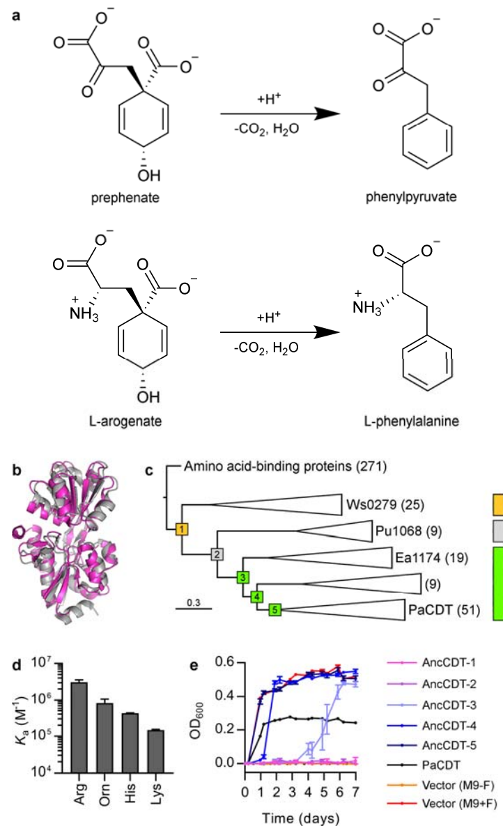
Figure 1. Functional evolution of CDT. a , Fragmentation reactions of prephenate and L-arogenate catalyzed by CDT. b , Structural similarity between PaCDT (grey; PDB: 3KBR) and Ws0279 (pink; PDB: 3K4U) (root-mean-square deviation 2.25 Å for backbone atoms). c , Condensed maximum-likelihood phylogeny of CDT homologs. The scale bar represents the mean number of substitutions per site. The five compressed clades are labeled with the corresponding number of sequences and the representative extant protein characterized in this work. The five ancestral nodes that were characterized experimentally (AncCDT-1 to AncCDT-5) are labeled and colored according to function (gold, amino acid binding; grey, binding of unknown solute; green, CDT). d , Affinity of AncCDT-1 for cationic amino acids, determined by ITC (Orn, L-ornithine). Results are mean \pm s.d. for two (Orn, Lys) or three (Arg, His) titrations. e , Growth of auxotrophic E. coli \Delta pheA cells complemented with ancestral proteins or PaCDT in selective M9–F media. Growth curves of empty vector transformants in selective M9–F media and unselective M9+F media are shown as negative and positive controls, respectively. Results are mean \pm s.e.m. for four biological replicates (AncCDT-5) or five biological replicates (otherwise).
