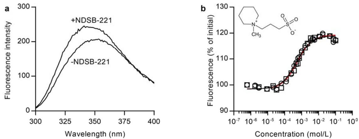
Extended Data Figure 5. NDSB-221 is a low-affinity ligand of Pu1068. a , Fluorescence spectrum of Pu1068 in the presence and absence of 10 mM NDSB-221, with an excitation wavelength of 280 nm. b , Fluorescence titration of Pu1068 with NDSB-221; peak fluorescence is plotted against ligand concentration. Two replicate titrations are shown. Fitting the data to a Boltzmann function gives a K_d of 530 \mu M and a maximum fluorescence change of 20%. The structure of NDSB-221 is inset.
