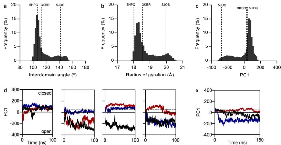
Extended Data Figure 10. Molecular dynamics simulations of PaCDT. a-c , Frequency histograms of the interdomain angle ( a ), the radius of gyration ( b ), and the projection onto the first principal component (PC1) ( c ) for individual PaCDT subunits in the eight simulations using the GROMOS 53a6 force field (1.08 \mu s simulation time). Each quantity can be used as a descriptor of the conformational change between the open and closed states of the protein. The corresponding values for the crystal structures of PaCDT (PDB: 5HPQ, 3KBR) and AncCDT-3(P188L) (PDB: 5JOS) are also shown. d-e , Projections of the trajectories of individual PaCDT subunits onto the PC1 axis. Each color represents a subunit of the PaCDT homotrimer. The dotted line represents the crystallographic conformation (5HPQ). ( d ) 4 \times 100 ns simulations initialized from 3KBR using the GROMOS 53a6 force field. ( e ) 1 \times 150 ns simulation initialized from 5HPQ using the OPLS3 force field.
