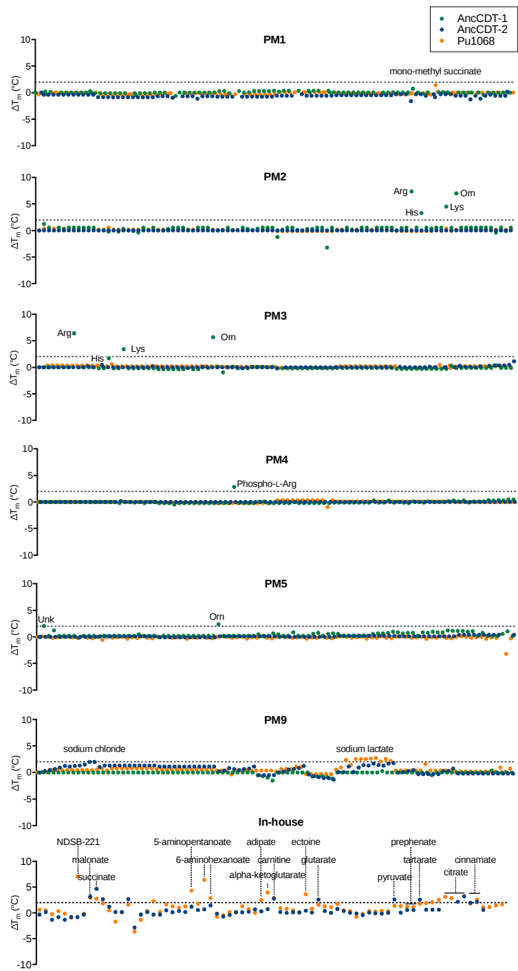
Extended Data Figure 4. Ligand screening of Pu1068 and AncCDT-2. DSF was used to screen Pu1068, AncCDT-2, and AncCDT-1 (as a positive control) against 650 different conditions from six proprietary screens from Biolog (PM1–5 and PM9) and an in-house screen comprised of various additional compounds. \Delta T_M values are given relative to a protein-only control. Compounds that produced a \Delta T_M greater than 2 °C are listed. No binding of prephenate, the substrate of CDT, was observed. Details of the screen compositions and ligand concentrations are provided in Supplementary Table 3 .
