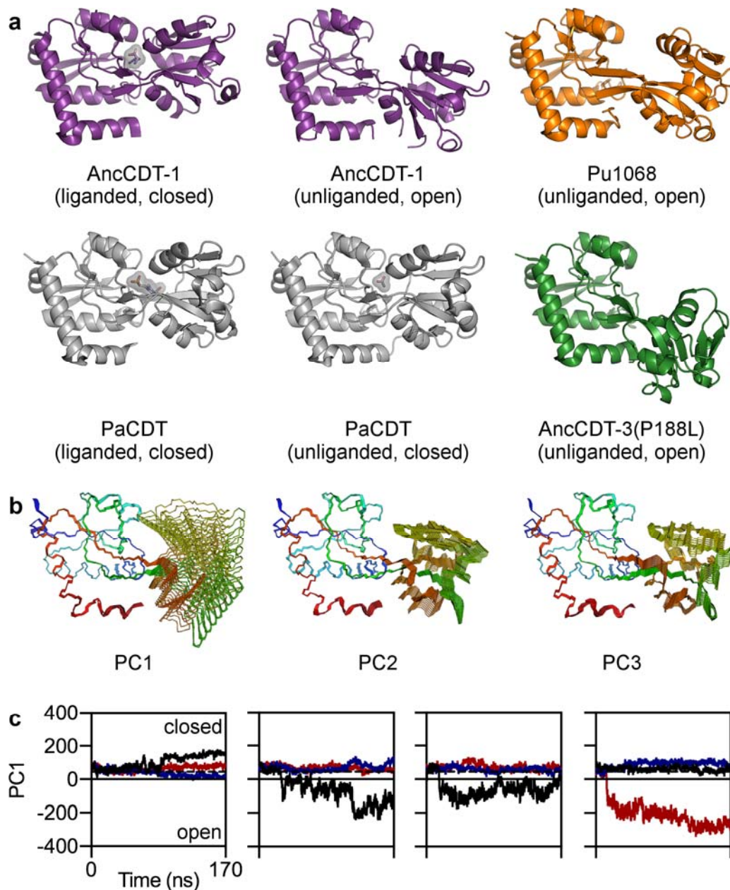
Figure 4. Structural dynamics of CDT. a , Open and closed structures of AncCDT-1, Pu1068, PaCDT, and AncCDT-3(P188L). Unusually, PaCDT adopts a closed structure in the absence of ligand. b , Principal component analysis of MD simulations of PaCDT. The structures illustrating the physical interpretation of the first three principal components (PCs) were generated by interpolating between structures at the extremities of each principal component axis. These motions represent hinge-bending and hinge-twisting motions typical of AABPs 18,19 . c , Open-closed conformational dynamics in 4 \times 170 ns simulations of PaCDT, initialized from the unliganded structure (PDB: 5HPQ) using the GROMOS 53a6 force field. Projections of the trajectories of individual PaCDT subunits onto the PC1 axis are shown. Each color represents a subunit of the PaCDT homotrimer. The dotted line represents the crystallographic conformation (PDB: 5HPQ).
