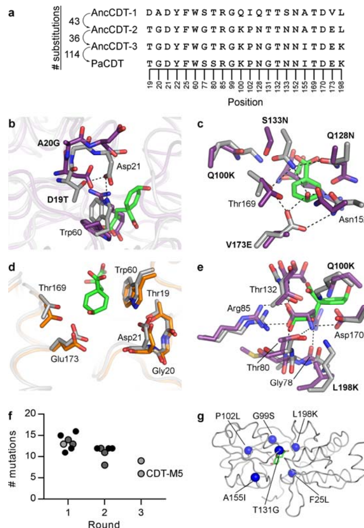
Figure 3. Structural and mutational basis for evolution of CDT activity. a , Multiple sequence alignment of ancestral proteins and PaCDT at positions important for CDT activity. The number of substitutions between each sequence in this evolutionary trajectory is shown. b-e , Comparison of AncCDT-1 (purple), Pu1068 (orange), and PaCDT (grey). Positions are labeled with the corresponding residue in AncCDT-1 and AncCDT-3, if conserved in both proteins, or with the corresponding substitution between the two proteins. b , The ancestral binding site was remodeled by a conformational change of Trp60. D19T introduces a hydrogen bond with Asp21, and A20G enables a conformation disfavored for non-glycine residues but necessary for the interaction between Thr19 and Asp21. c , Functionalization of the ancestral binding site introduced the general acid Glu173 and residues required for substrate binding and transition state stabilization. d , Structural similarities between Pu1068 and PaCDT. The two domains of Pu1068 were superimposed separately on the structure of PaCDT. e , CDT inherited the \alpha -amino acid-binding motif from AncCDT-1, with two substitutions (Q100K, L198K) that also enable binding of the \alpha -keto acid prephenate. f , Introduction of CDT activity into AncCDT-2 by directed evolution. Each point represents a unique clone, and the color gives a qualitative indication of activity (black, high activity; dark grey, moderate activity; light grey, low activity). See also Extended Data Figure 8 . g , Positions of six substitutions sufficient to introduce CDT activity into AncCDT-2. F25L, G99S, P102L and A155I are located in the second or third shells of the active site.
