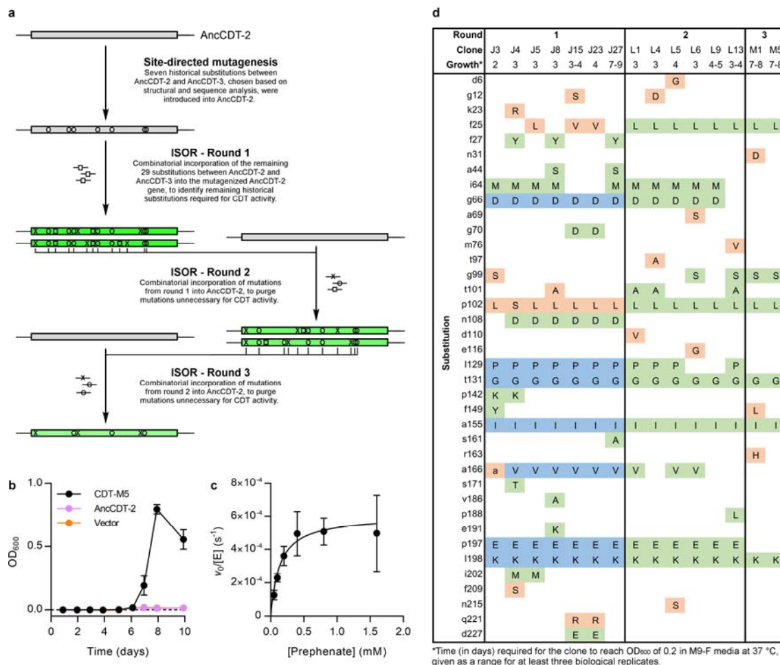
Extended Data Figure 8. Directed evolution of AncCDT-2. a , Overview of the strategy used for directed evolution of AncCDT-2. b , Complementation of auxotrophic E. coli \Delta pheA cells in selective M9-F media by CDT-M5 (mean \pm s.e.m., three biological replicates). AncCDT-2 and empty vector transformants were used as negative controls. c , Michaelis-Menten plot for CDT-M5 (mean \pm s.d. of 3 – 8 technical replicates). d , Sequences of AncCDT-2 variants with CDT activity, isolated by genetic selection of ISOR libraries. Amino acid substitutions in blue originated from the template gene (via site-directed mutagenesis), substitutions in green were encoded in oligonucleotides, and substitutions in orange were acquired randomly.
