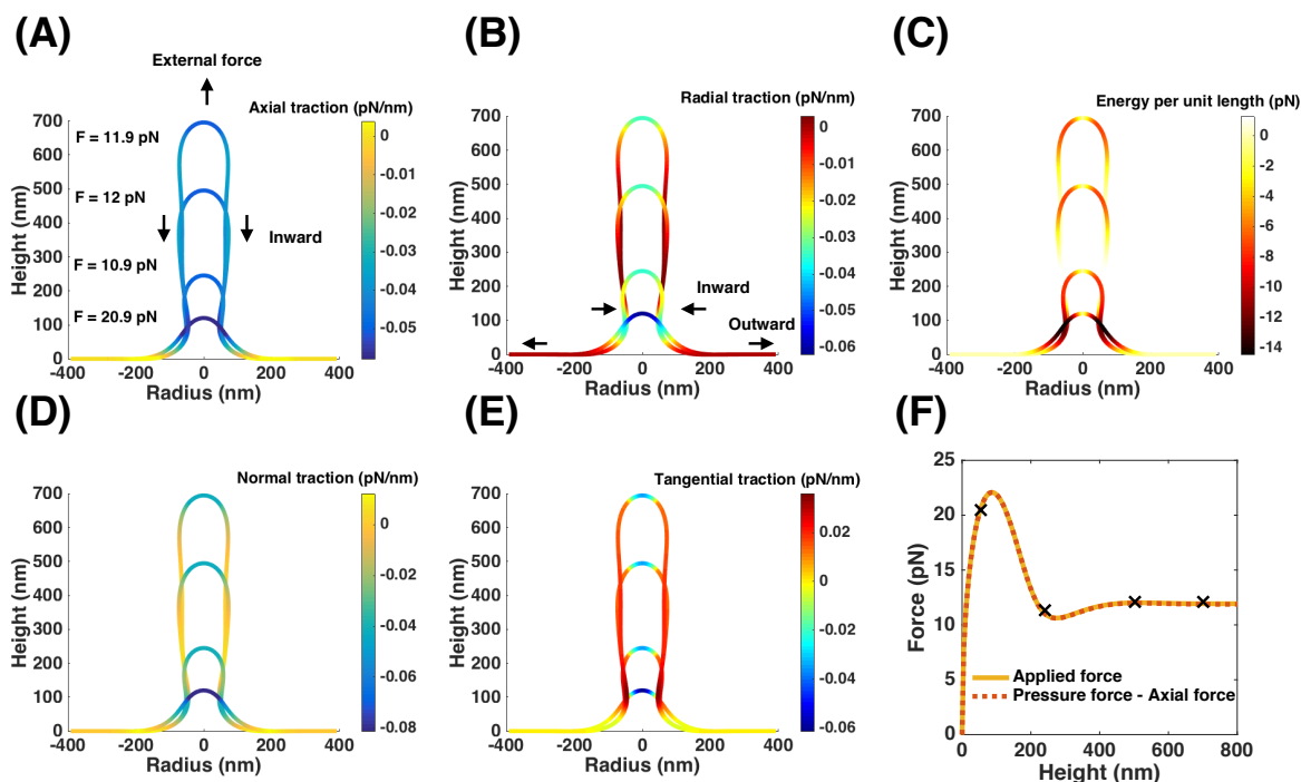
Figure S2: Tether pulling simulation for the pressure of 0.3 kPa, bending modulus 320 pN · nm, no surface tension at the boundary ( \lambda_0 = 0 ), and a point force. (A) Axial traction distribution along the tether. (B) Radial traction distribution. We find a negative value at the neck and a positive value at the base. (C) Energy per unit length (Eq. 6) plotted along the shapes. We observe a large value at the neck - predicting an ‘effective’ line tension of 11 pN for a tether of height 700 nm. (D) Normal traction distribution. It is large and negative over the area of applied force. (E) Tangential traction distribution. (F) Applied force and the difference between the calculated pressure and axial force (Eq. S29) plotted as a function of tether height.
