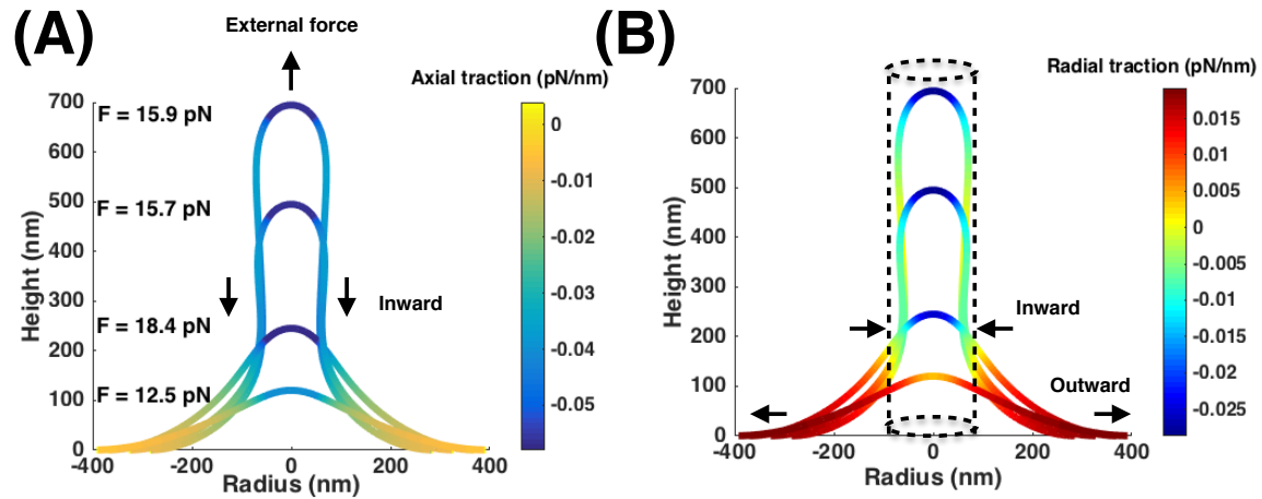
Figure S1: Axial and radial traction (Eqs. S28b, S28a) distribution plotted along the same membrane shapes as in Fig. 3A–C. (A) Axial traction distribution. The axial traction is constant along the tube. (B) Radial traction distribution. The dotted line is the stable cylindrical geometry.
