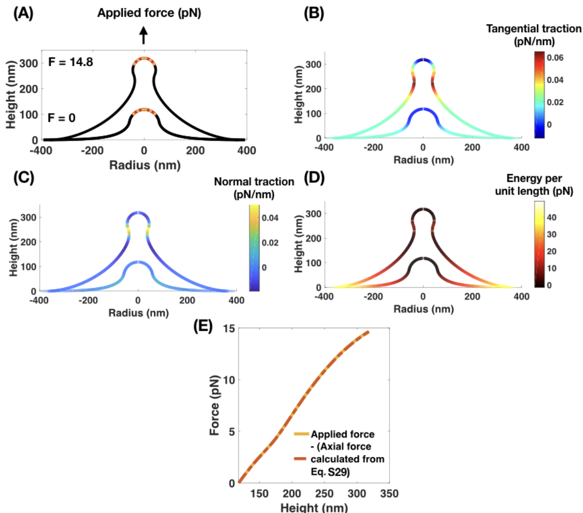
Figure S9: Application of axial forces (brown) onto a U-shaped bud covered by a protein coat (red). Spontaneous curvature magnitude C = -0.02 \text{ nm}^{-1} , area of spontaneous curvature field A = 17,593 \text{ nm}^2 , bending modulus \kappa = 320 \text{ pN} \cdot \text{nm} and surface tension at the edge \lambda_0 = 0.02 \text{ pN/nm} . Here, axial forces are applied such that there is only an upward force over the protein coat. (A) Initial and final membrane shapes obtained. Force required is smaller than Fig. S8. (B) Tangential traction distribution along the membrane shapes in (A). (C) Normal traction distribution along the membrane shapes in (A). (D) Energy per unit length along the membrane shapes in (A). (E) Force match obtained between applied force and negative of axial force calculated using Eq. S29. Here, axial force is calculate at the base of the membrane. The same match can be obtained at the edge of the protein coat.
