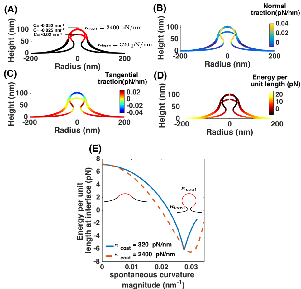
Figure S5: Analysis of membrane budding due to protein-induced spontaneous curvature with a rigid coat. Simulations for Fig. 5 is repeated for \kappa_{\text{coat}} = 2400 \text{ pN/nm} and \kappa = 320 \text{ pN/nm} . (A) Membrane shapes for same three spontaneous curvature as Fig. 5 A. (B) Normal traction along the membrane for the shapes shown in (A). (C) Tangential traction distribution (D) Energy per unit length distribution for the chosen shapes. (E) Energy per unit length at the edge of the edge of the spontaneous curvature field as a function of spontaneous curvature for the homogeneous membrane in Fig. 5 (blue solid line) and a rigid protein coat (red dashed line). In large values of spontaneous curvature ( \Omega -shaped bud) the average difference between the line tension magnitudes is almost 4 pN.
