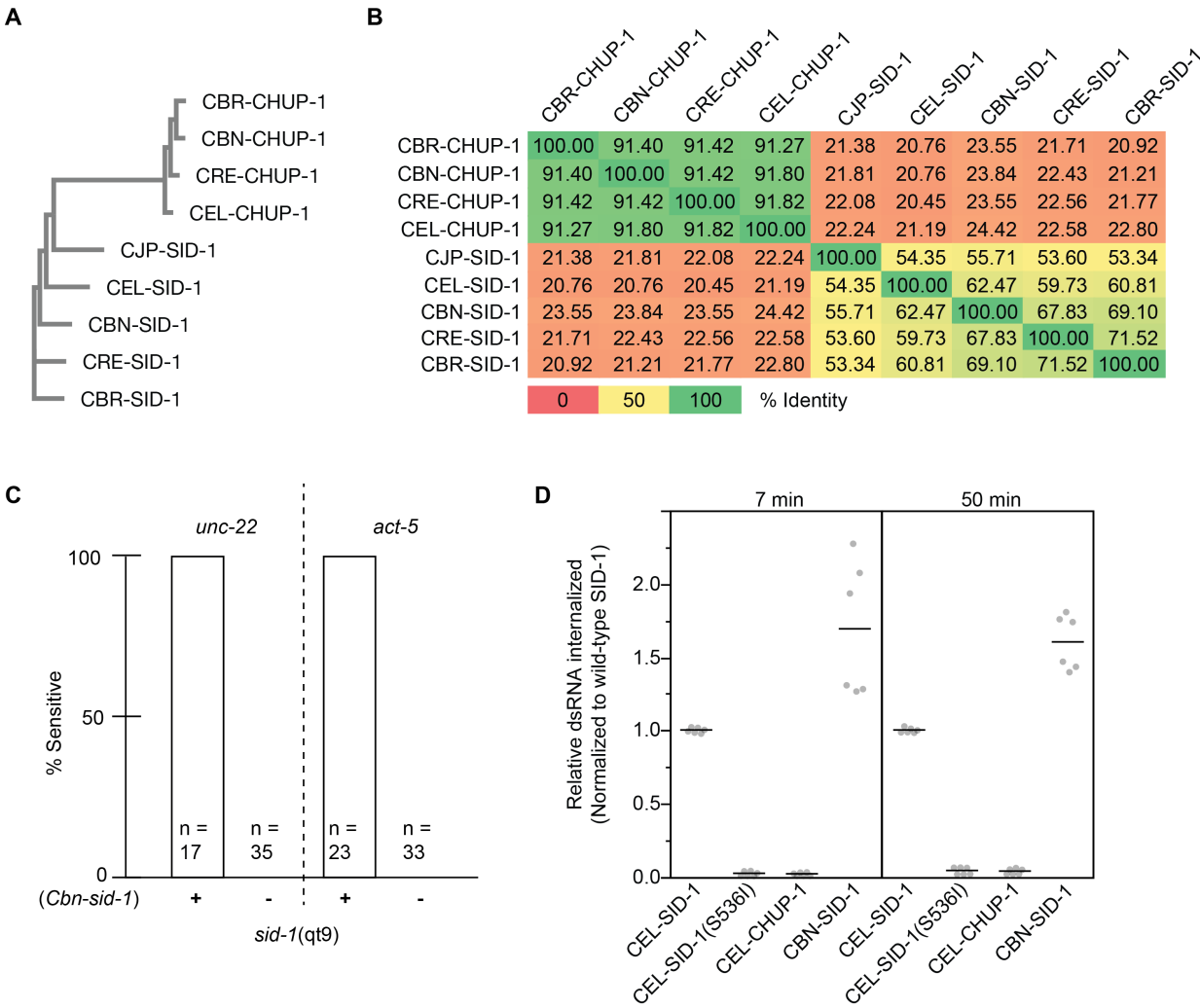
Figure 1. Sequence and functional relationships among SID-1 homologs. (A) Phylogenetic tree of nine Caenorhabditis SID-1 homologs (MUSCLE v3.8). (B) Pairwise percent identity heat matrix of homologs. (C) sid-1(qt9) animals with or without an extrachromosomal array containing a cbn-sid-1 genomic fragment were tested for RNAi sensitivity on unc-22 or act-5 RNAi food. (D) Internalization of 32 P-labeled 500 bp dsRNA into Drosophila S2 cells expressing the indicated SID-1 constructs. Line represents mean value of 2 biological replicates.
