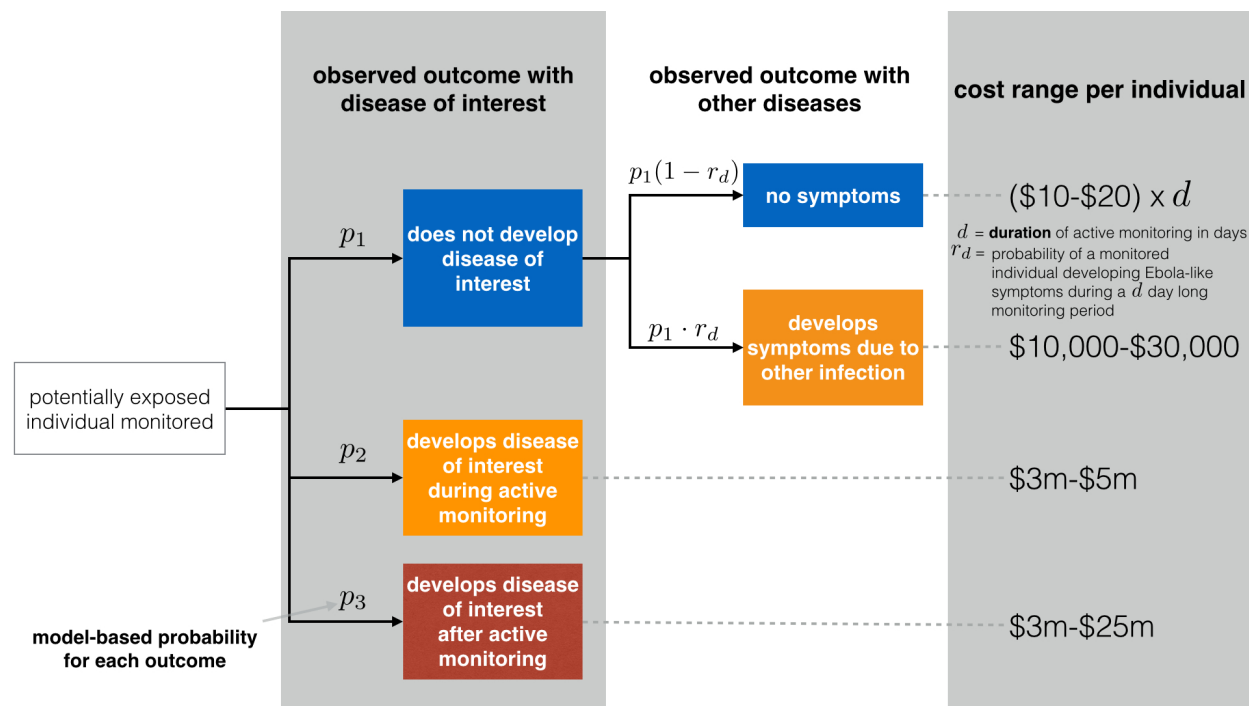
Figure 1 Model schematic representing four outcome scenarios for a person under active monitoring. Estimated costs shown are based on published costs(23) as well as new data from DOHMH and Bellevue Hospital in NYC. Details on the model formulation are available in Supplemental Table 3. Our model uses probabilities to calculate the likelihood of each of the possible model outcomes. Additionally, we estimate the probability that an individual who does not develop the disease of interest develops symptomatic illness necessitating hospitalization to rule-out the disease of interest. (See Supplemental Text for details.)
