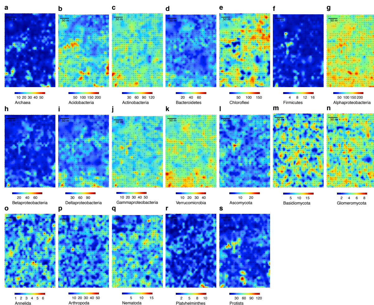
Figure 2. Spatial distribution of OTU diversity per focal clade. The colour scale is expressed as effective numbers of OTUs (exponential Shannon diversity index) for archaea (a), bacterial clades (b-k) and eukaryotic clades (l-s). Maps were obtained by ordinary kriging. Grey dots represent the samples available for each clade.
