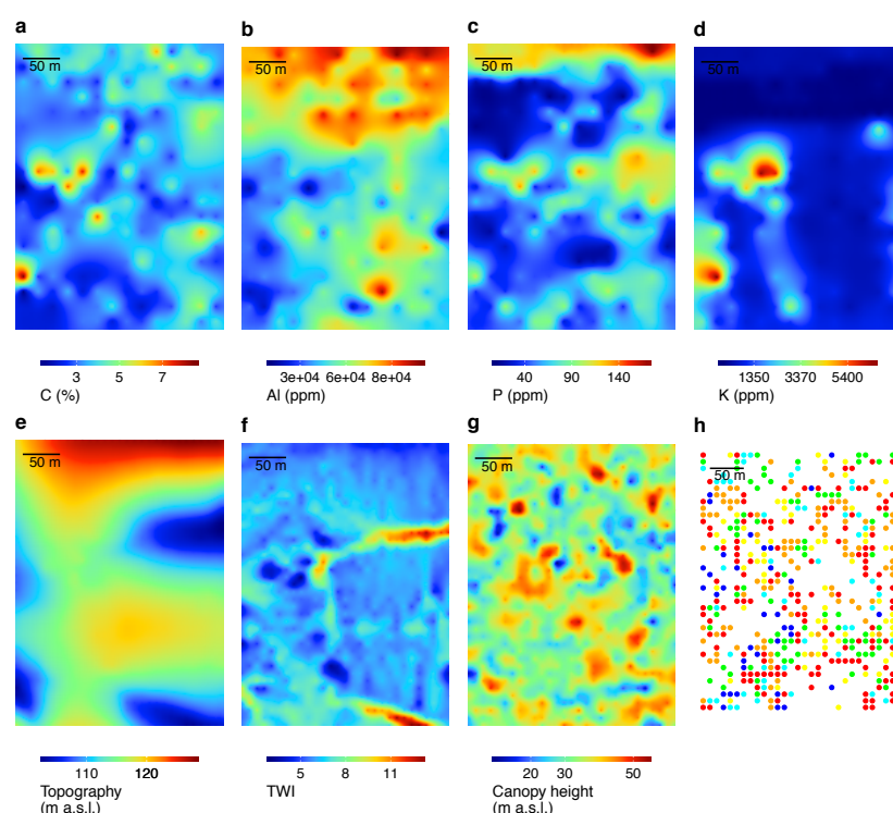
Figure 1. Maps of environmental characteristics in the 12 ha plot. a-d) Soil content in Carbon, Aluminium, Phosphorous and Potassium. e) site topography, f) soil wetness (TWI index, unitless) and g) canopy height as inferred from LiDAR data. h) Distribution of the most dominant plant genus found in each soil sample as inferred from the plant molecular dataset. Only the six most frequent dominant genera are shown: red: Apocynaceae; orange: Andira; yellow: Ingeae; green: Brosimum; lightblue: Sapotaceae; blue: Drypetes. x/y axes are not shown for representation purposes and range between 10-290 and 10-390 meters respectively.
