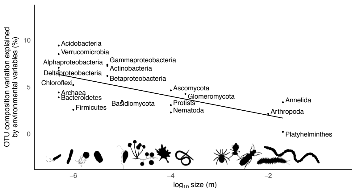
Figure 4. Variation of OTU composition explained by environmental variables according to organism propagule size. The variation ( R^2_{adj} statistics) includes pure plants and abiotic effects as well as their combined effect with spatial variables. The negative relationship between organism propagule size and the variance explained by environmental effects is significant (Pearson's r = -0.67 , p = 0.002 ).
