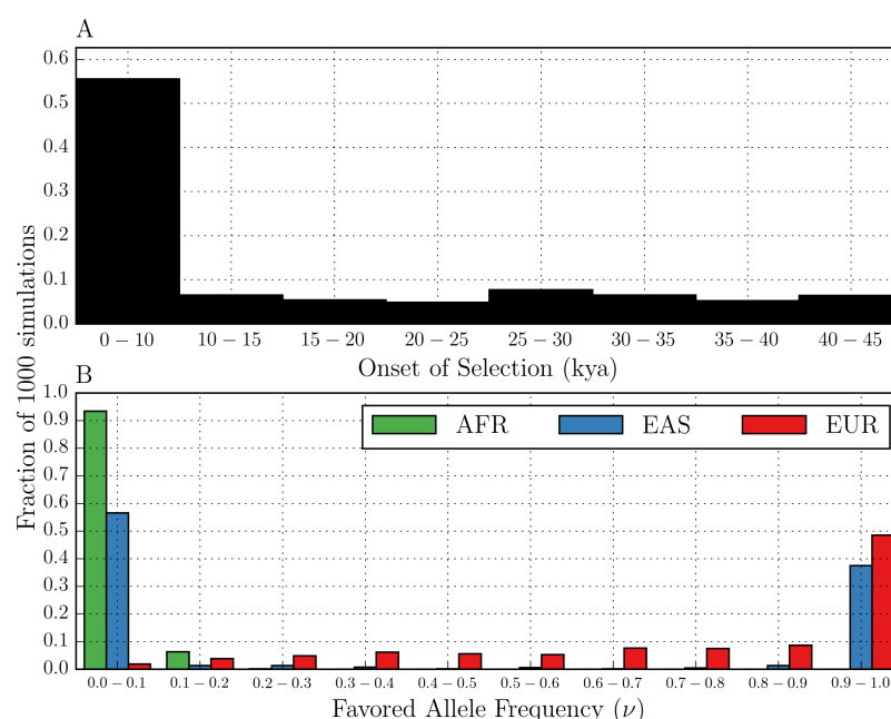
Figure S21: Simulation of Selection on Human Demography. We simulated 1000 selective sweeps on 5Mbp region based on the human demography model described in Fig. S20, and with selection coefficient s = 0.05 and starting favored allele frequency \nu_0 = 0.001 . A) The selection happens in a random time, after the out of Africa in the lineage of EUR population (as the target population). B) When the onset of selection is before split of EUR and EAS ( > 23 kya), both (EUR and EAS) are under selection.
