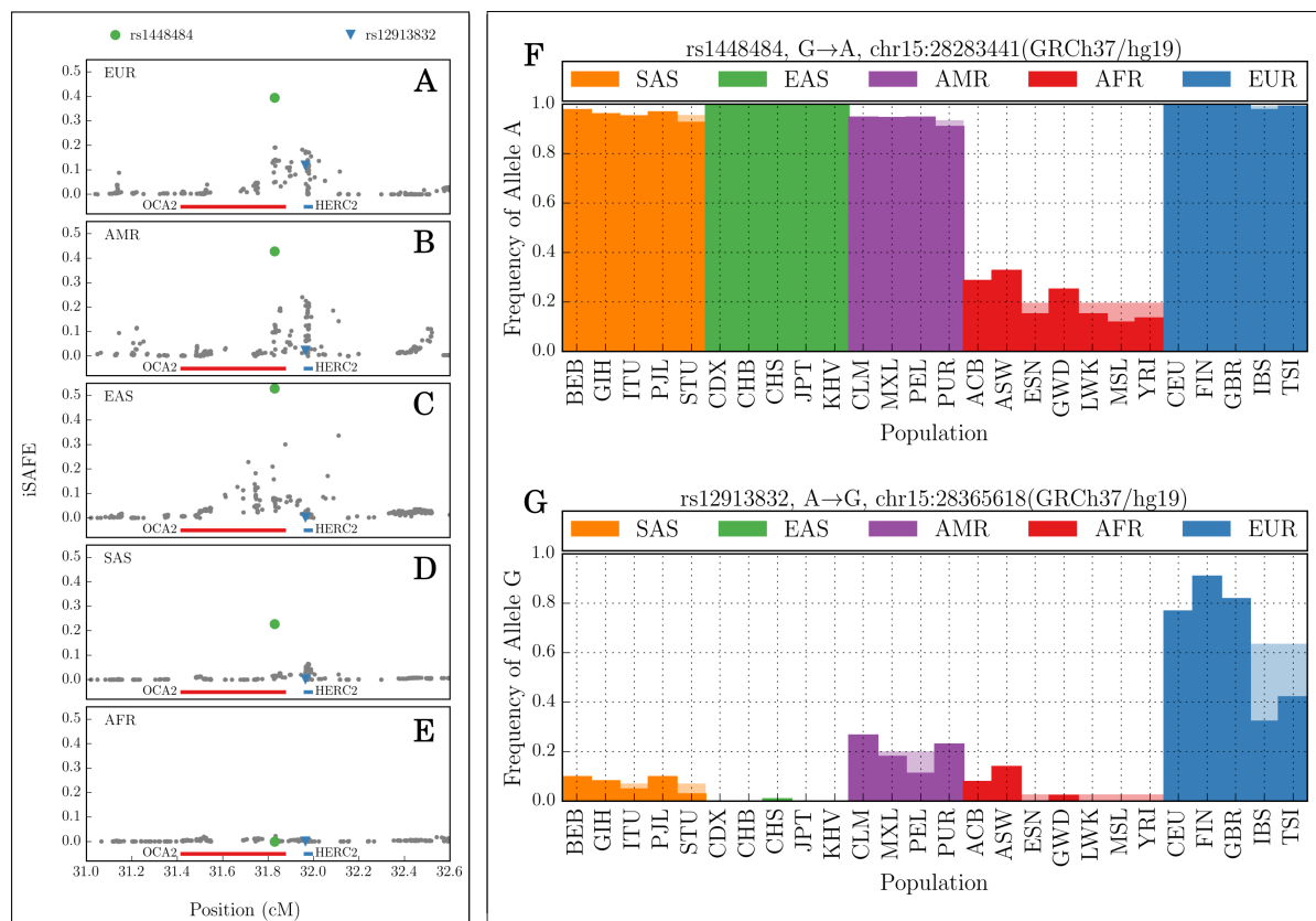
Figure S25: iSAFE on OCA2-HERC2. The mutation rs1448484 is the iSAFE top rank mutation in all the population of 1000GP except African that doesn't show any signal of selection in this region. rs12913832 is a candidate favored mutation for the selection in European, proposed by 9 . Table S2 provides iSAFE rank of some other candidate mutations associated with pigmentation 28 .
