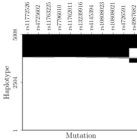
Figure S28: SNP matrix of TRPV6 top candidates. Haplotypes of top 10 iSAFE mutations, and the proposed mutation (rs4987682) by 26 , in 5Mbp around TRPV6 in 2504 \times 2 haplotypes of 1000GP are shown. These mutations are sorted by their iSAFE rank from left to right. iSAFE top 10 mutations span a 9kbp region(chr7:142476441-142485399, GRCh37/hg19). White is derived and black is ancestral allele.
