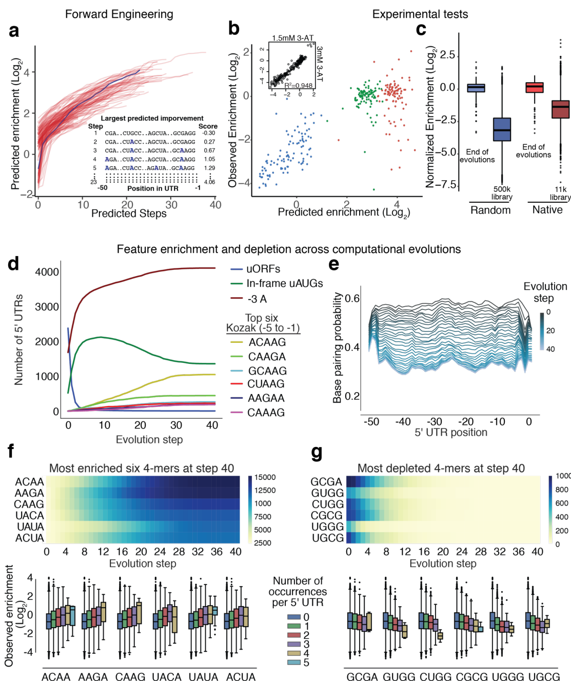
Figure 4 - Model-guided optimization of 5000 random sequences.
