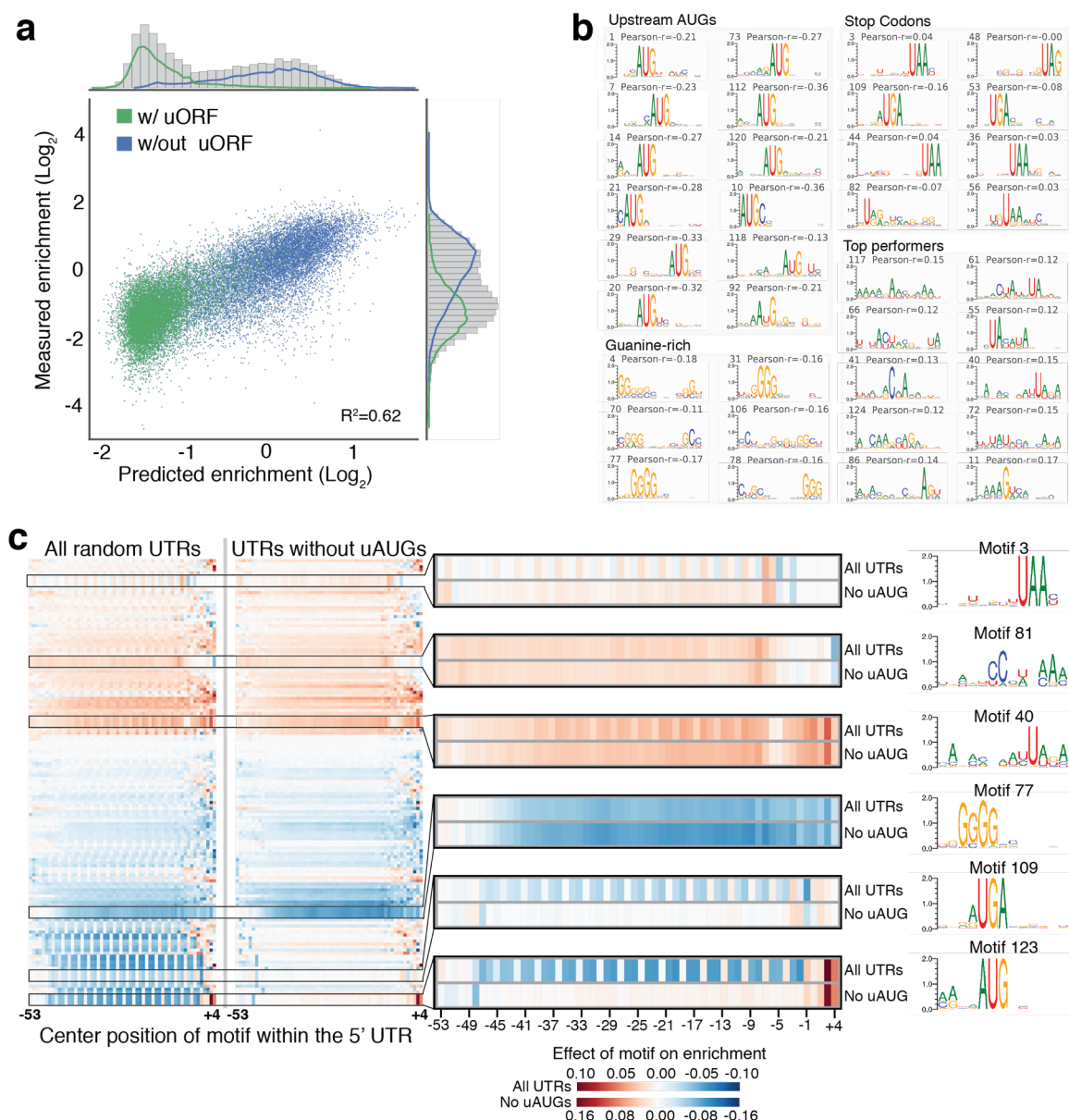
Figure 2 - A convolutional neural network approach to model random 5' UTR sequences.
