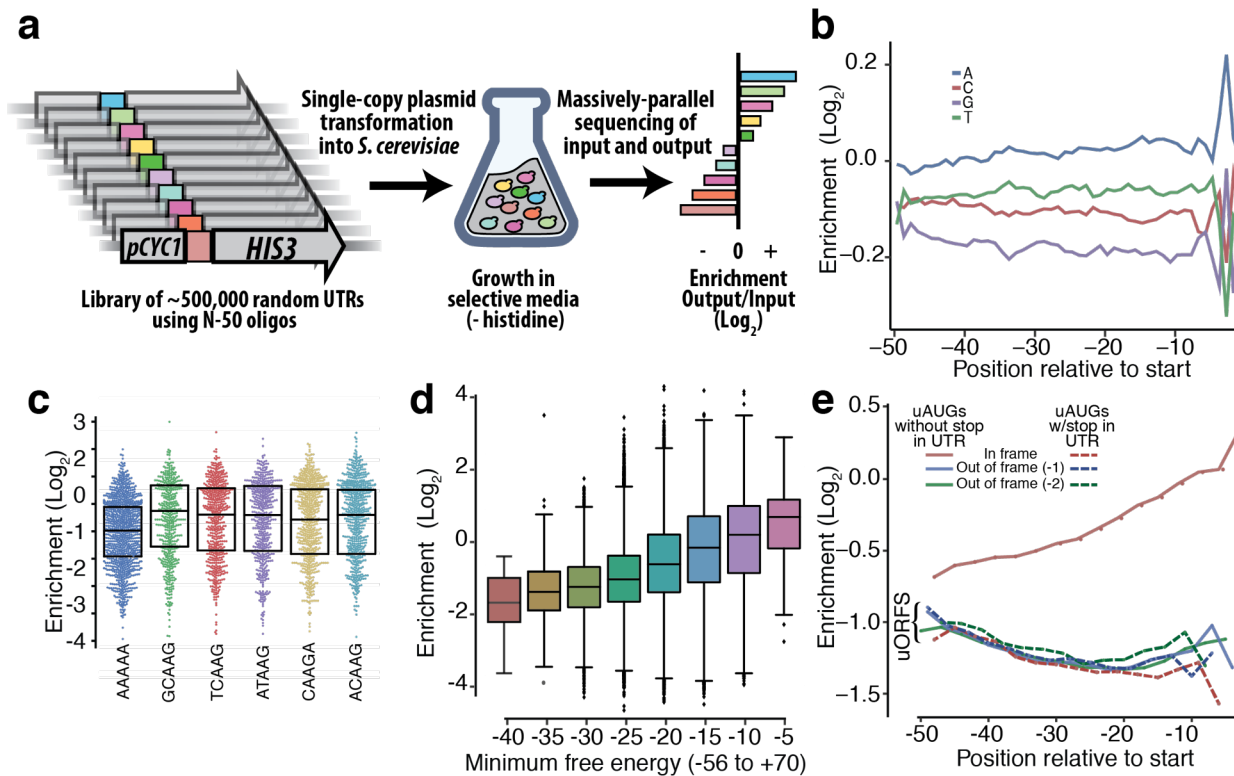
Figure 1 - Experimental design and biological discovery.
