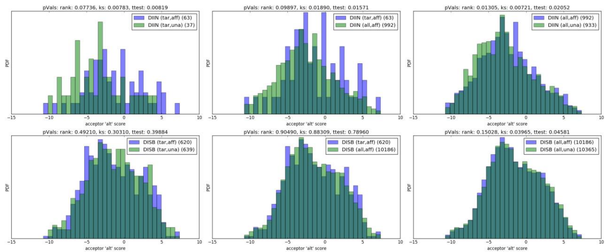
Figure S6. acceptor 'alt' score distributions
