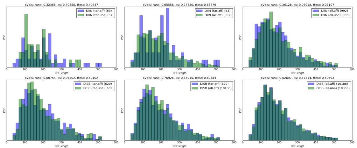
Figure S5. ORF length distributions
