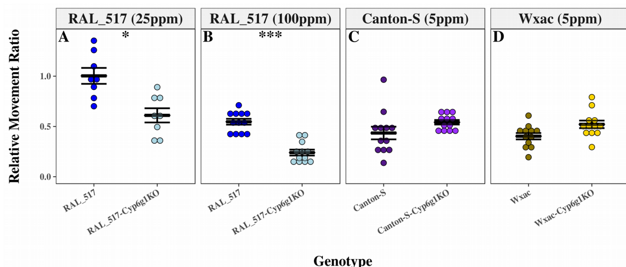
Figure 4- Imidacloprid Resistance in Cyp6g1KO Backgrounds:
