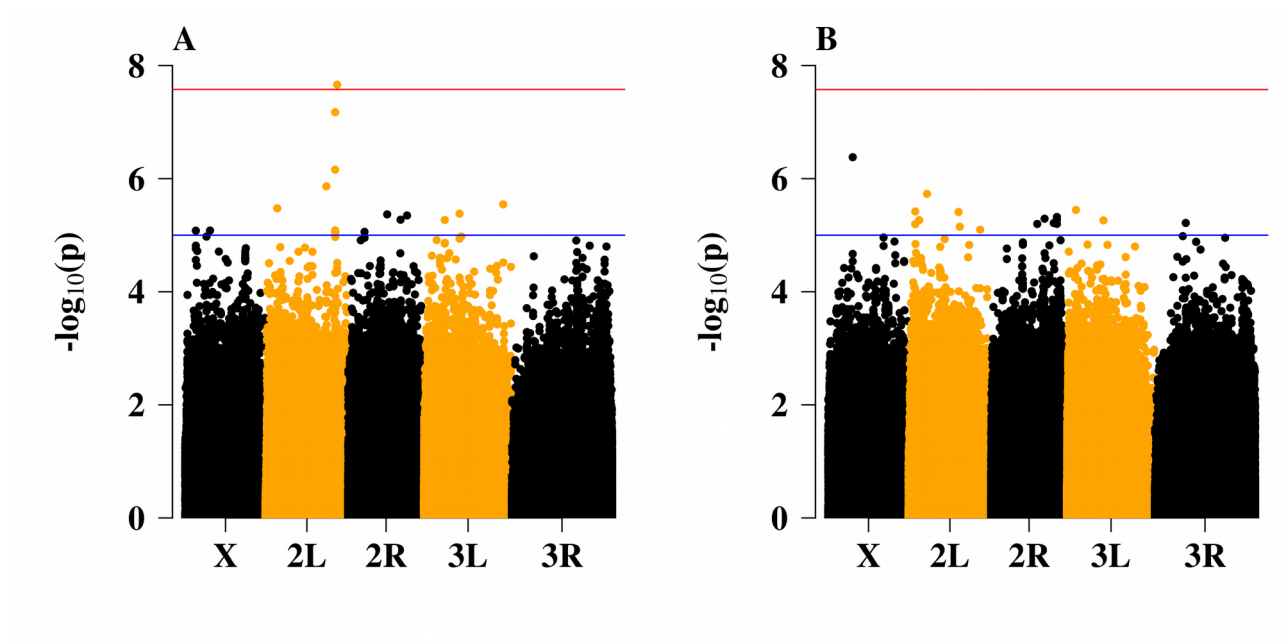
Figure S4- Manhattan Plots:
