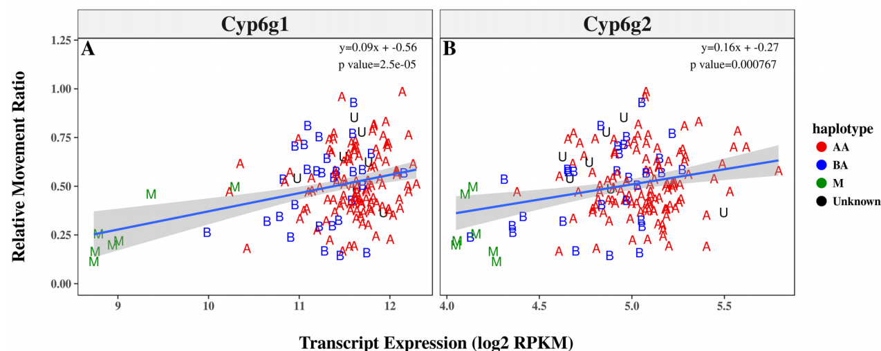
Figure 3- Transcriptional Association of Cyp6g1 and Cyp6g2:
