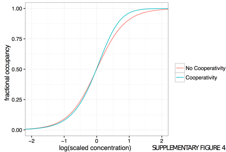
Supplementary Figure 4: Cooperativity between TFs results in steeper binding curves. The predicted fractional TF occupancy (y axis) for a given concentration of the TF (x axis), when the concentration of the cooperatively-interacting TF is constant. The two binding curves are aligned at 50% occupancy to emphasize the differences in the slopes. Modeling was done as described in Methods .
