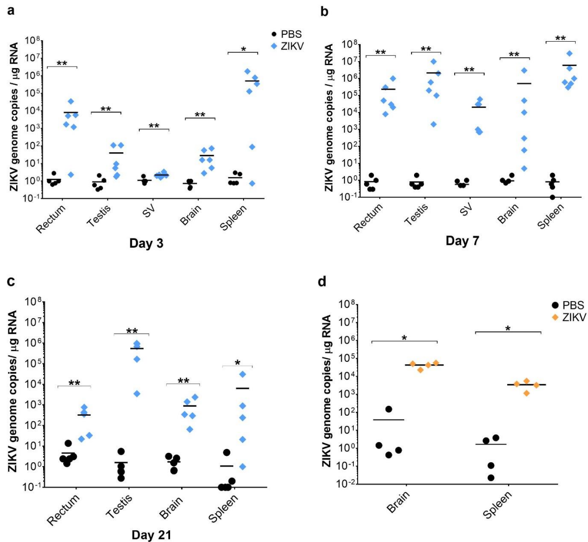
Figure 2. Tissue viral load following rectal and subcutaneous routes of ZIKV inoculation. Graphs depict ZIKV genome copies detected by RT-qPCR in various tissues at 3 dpi (A), 7 dpi (B), and 21 dpi (C). Each symbol corresponds to data from an individual mouse. n=5-6 mice per group. (D) Viral load in the spleen and brain at 6 days post-subcutaneous infection with ZIKV. n=4 mice per group. Two-tailed unpaired, non-parametric Mann-Whitney tests were conducted, where *p < 0.05 and **p < 0.001.
