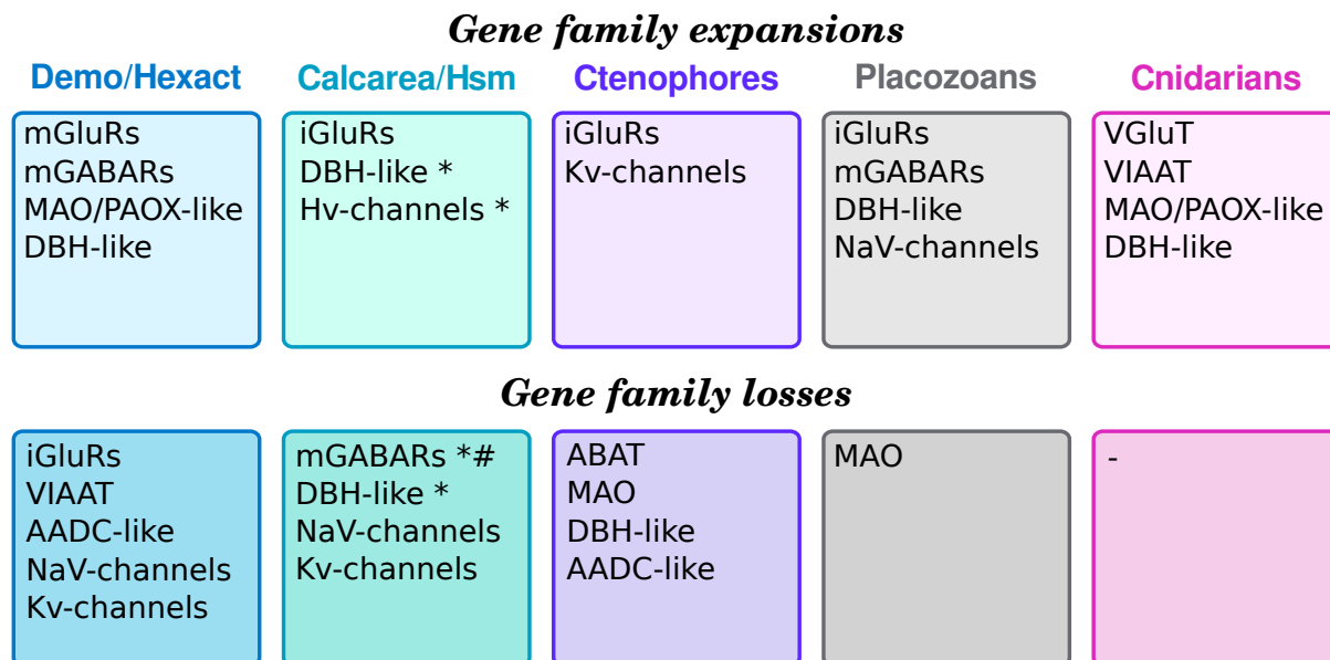
Figure 6: Summary of gene expansions and losses
