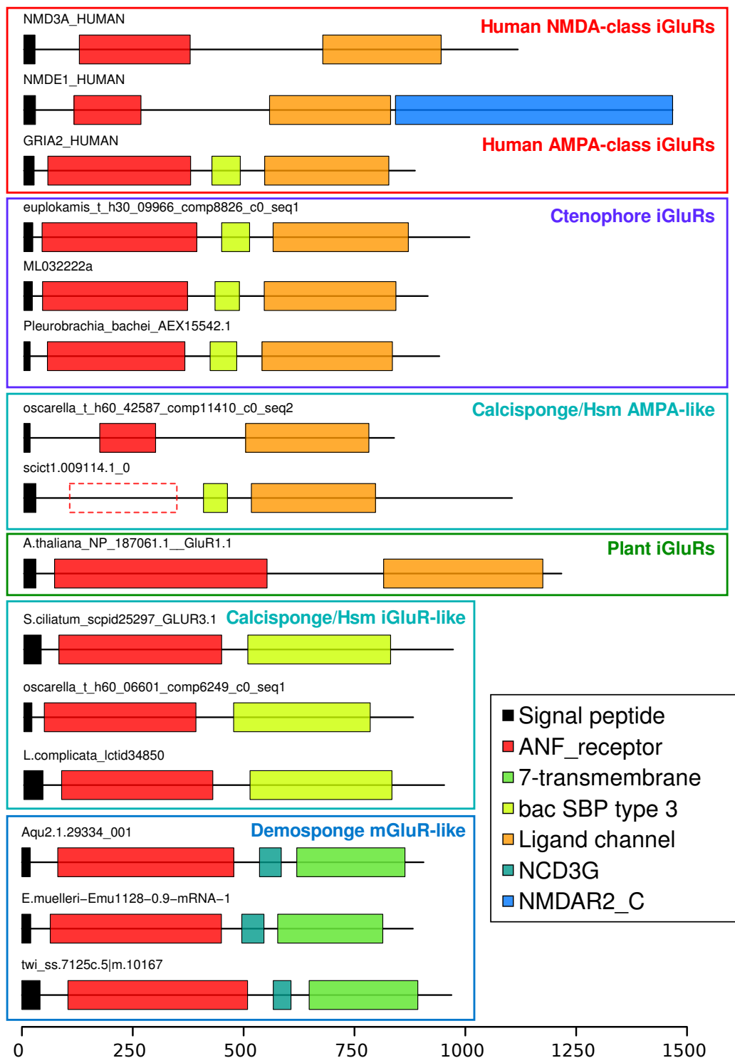
Supplemental Figure 13: Domain organization of ionotropic glutamate receptors across metazoans
