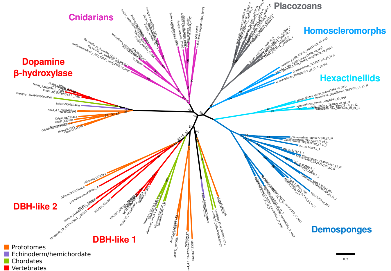
Supplemental Figure 7: Dopamine \beta -hydroxylase homologs across metazoans Tree of DBH and DBH-like proteins across all metazoan groups, generated with RAXML using the PROT GAMMALG model. Bootstrap values are 100 unless otherwise shown.
