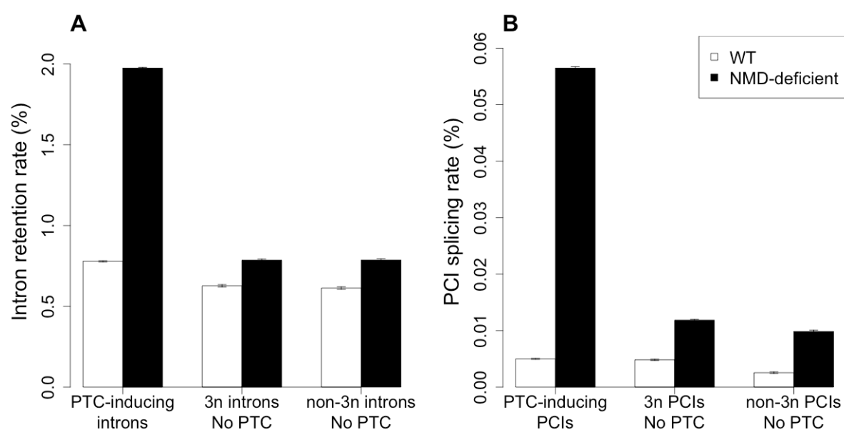
Figure 2: Impact of NMD on observed AS rates. AS events (IR or cryptic intron splicing) are classified into three groups according to their NMD-visibility: PTC-inducing events (i.e. NMD-visible); events that do not introduce frameshift or PTC
