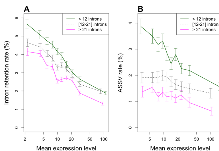
Figure 5: Relationship between AS rate, expression level and number of introns in human genes. (A) IR rate ( N=118,703 introns). (B) ASSV rate ( N=102,697 introns). In both panels, introns were first classified into three groups of equal sample size, according to the number of introns of the genes in which they are located (genes with < 12 introns, genes with 12 to 21 introns, genes with > 21 introns), and then further grouped into ten bins of equal sample size, according to gene expression levels. We computed the average AS rate (IR or ASSV) over all introns within each bin. Error bars represent the 95% confidence interval of the mean. Expression levels (RPKM, averaged over the 52 samples) are represented in log scale
