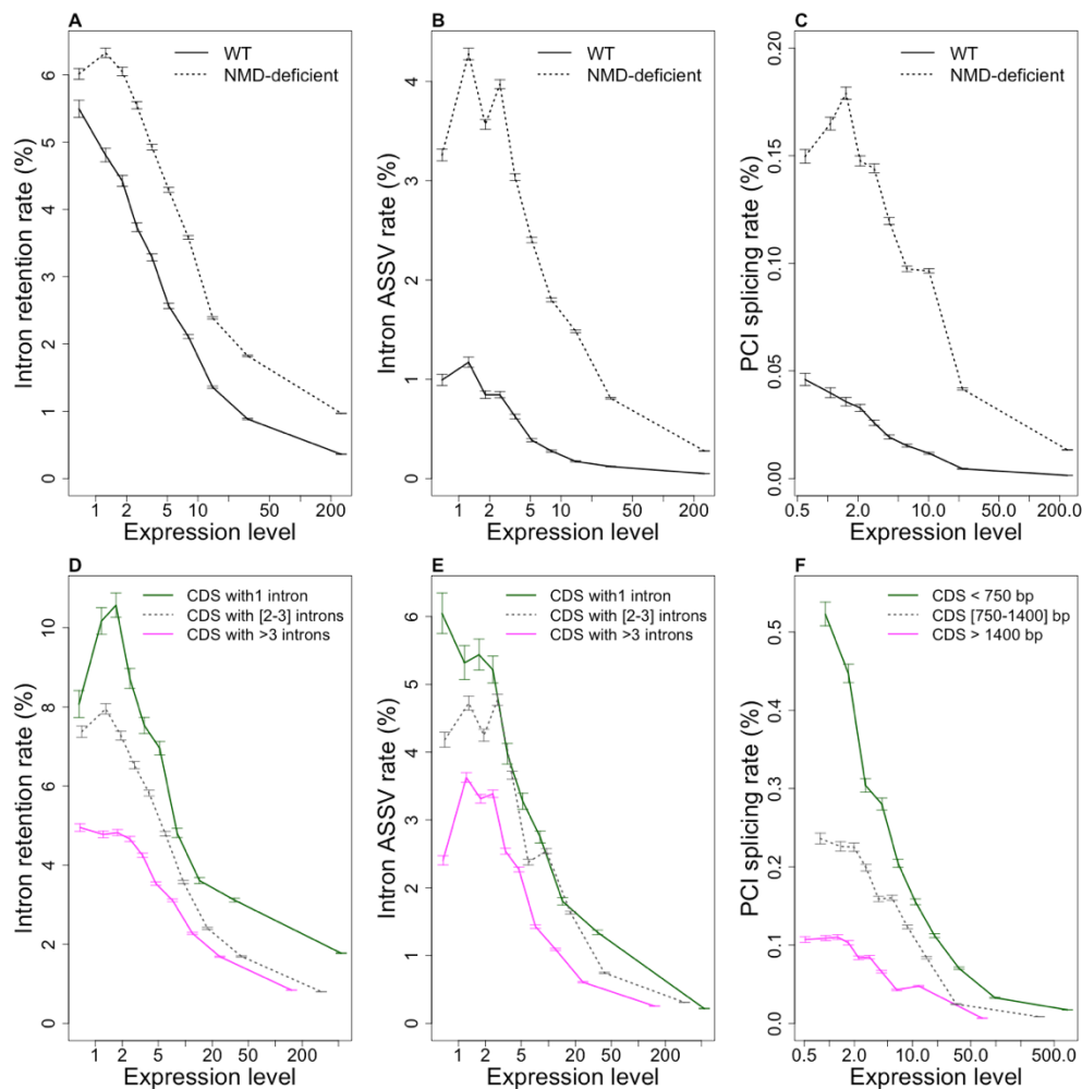
Figure 3: Relationship between AS rate and gene features: expression level, number of introns or length of coding regions. Introns (N= 65,159) and PCIs (N= 1,383,067) were classified into ten bins of equal sample size, according to gene expression levels in WT cells. The AS rate was computed globally within each bin, as the proportion of AS reads among all reads spanning introns (or PCIs) from that bin. Error bars represent the 95% confidence interval of this proportion. (A) IR rate; (B) ASSV rate; (C) Rate of splicing at potential cryptic introns. (D,E) same as (A,B), but introns were first classified into three bins, according to the number of introns of the gene in which they are located: genes with 1 intron (N=5,606 introns), genes with 2 to 3 introns (N=24,452 introns), genes with > 3 introns (N=35,101 introns). (F) same as (C), but PCIs were first classified into three bins, according to the length of the coding region (CDS) in which they are located: CDS < 750 bp (N=169,030 PCIs), CDS from 750 to 1400 bp (N=406,460 PCIs), CDS > 1400 bp (N=807,577 PCIs). (A,B,C): AS rates were measured in normal cells (WT, black line) and in NMD-deficient cells (dashed line). (D,E,F): AS rates were measured in NMD-deficient cells. Expression levels (RPKM) are represented in log scale.
