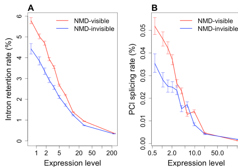
Figure 4: Relationship between AS rate and expression level, for NMD-visible or NMD-invisible AS events. (A) Introns were first classified into two groups according to their NMD-visibility in case of retention events ( N=52,163 NMD-visible introns, in red, and N=12,996 NMD-invisible introns, in blue), and then further grouped into ten bins of equal sample size, according to gene expression levels in WT cells. IR rates (in WT cells) were measured globally in each bin. Error bars represent the 95% confidence interval of the proportion of AS reads. (B) Same as (A), but for the splicing of PCIs: N=882,579 NMD-visible PCIs, and N=500,488 NMD-invisible PCIs. Expression levels (RPKM) are represented in log scale.
