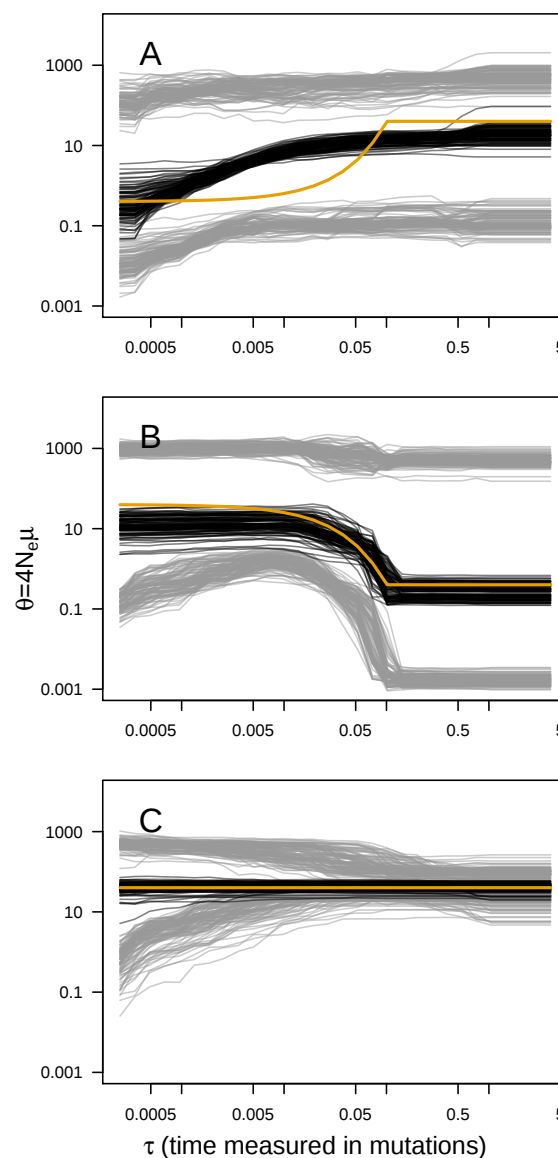
Figure 1. ABC Skyline plots: simulations. Superimposed skyline plots (median in black, and 95%HPD interval in grey of the posterior probability distribution for \theta(t) ) from 100 replicates for example (A) contraction ( \theta_0 = 0.4 , \theta_1 = 40 , \tau = 0.1 ), (B) expansion ( \theta_0 = 40 , \theta_1 = 0.4 , \tau = 0.1 ) and (C) constant size ( \theta = 40 ) scenarios with mutational model P_{GSM} = 0.22 . Simulation of 30 loci sampled at 50 diploid individuals. True demography is shown in orange. Note that present is at \tau = 0 (left).
