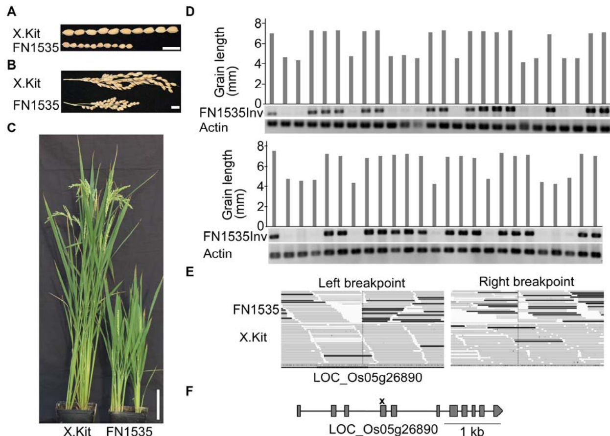
Figure 6. An Inversion Cosegregates with the Short-Grain Phenotype in Line FN1535.
