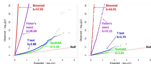
Fig. 1. Comparing ASE testing methods in LCLs from Tewhey et al. QQplot depicting the p -value distributions from testing for ASE using four different methods in LCLs with all SNPs (Left) or SNPs predicted to not have any regulatory effect (non-effect SNPs, Right). \lambda measures genomic inflation deviation from the uniform.
