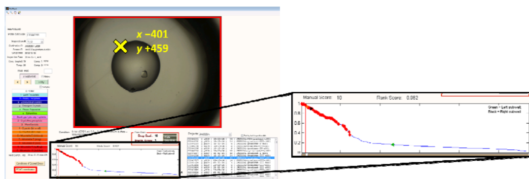
Figure 2 The TeXRRank interface showing a crystallisation drop containing a single JMJD2D crystal. Clicking a location records the acoustic dispensing target (yellow 'X' and x y coordinates have been added for clarity). Expanded section shows the ranked plot of crystal images.
