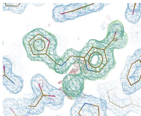
Figure 4 Electron density maps showing bound KDOAM16 ( \sigma_A -weighted 2mF_o - DF_c : blue, 1.4 \sigma , and mF_o - DF_c : red/green, \pm 3 \sigma , 1.5 \text{ \AA} resolution) calculated from refinement prior to including the ligand in the model.
