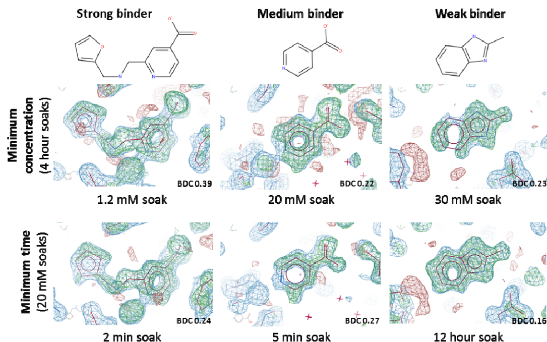
Figure 9 Electron density maps (PanDDA maps: event maps, blue, 2 \sigma , Z-maps: green/red, \pm 3 , 1.3–1.4 Å resolution) from the minimum experimental conditions (time or concentration series) required to detect ligand binding. The PanDDA reported background density correction (BDC) values are shown (Pearce et al. , 2016).
