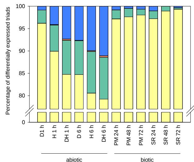
Figure 5: Response of differentially expressed (DE) triads to stress treatments according to the number and pattern of DE homoeologs. Triads were classified as having one homoeolog DE (yellow), two homoeologs DE with same direction of change (green), three homoeologs DE with same direction of change (orange), or opposite direction of change between DE homoeologs (blue). The stresses applied were drought (D), heat (H), drought and heat combined (DH), powdery mildew (PM) and stripe rust (SR), with the duration of stress application indicated in hours (h).
