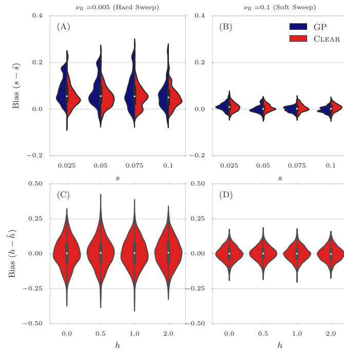
Fig S4: Distribution of bias for 30x coverage.
