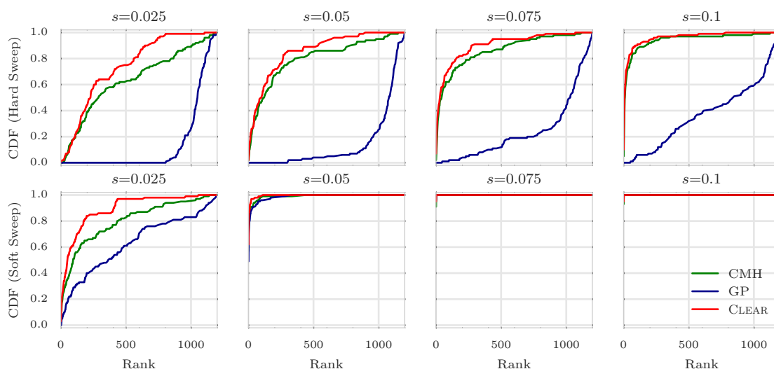
Fig 5: Ranking performance for 100 \times coverage.
