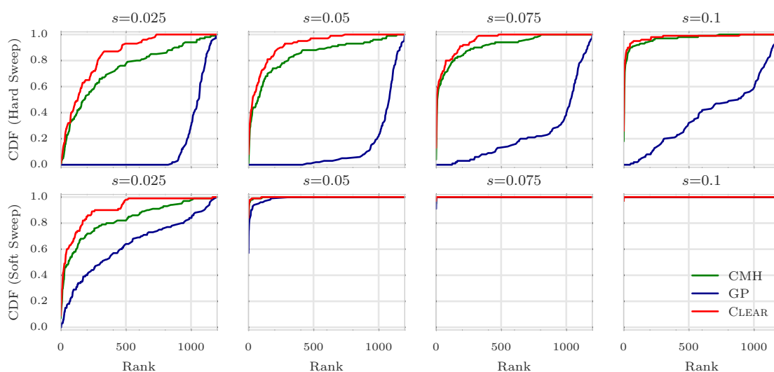
Fig S7: Ranking performance for 300 \times coverage.
