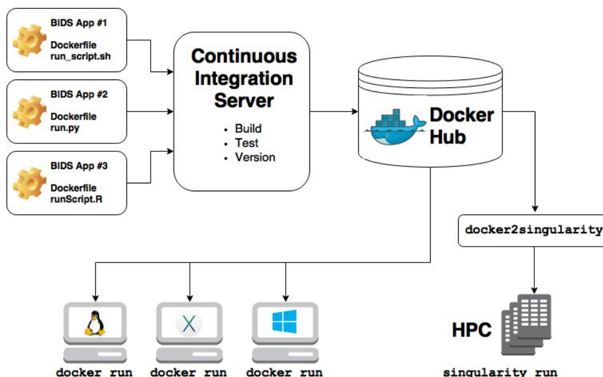
Figure 1. Overview of the creation and use of BIDS Apps. The source code of each App is stored in separate GitHub repository. Each repository is connected to a Continuous Integration server responsible for building testing and deploying the corresponding App. For every new release of an App, a new container image is deposited in Docker Hub. Users can directly download and run the BIDS Apps container images either directly using Docker on any Windows, Mac, and Linux machine or convert them to Singularity and run them on an HPC.
