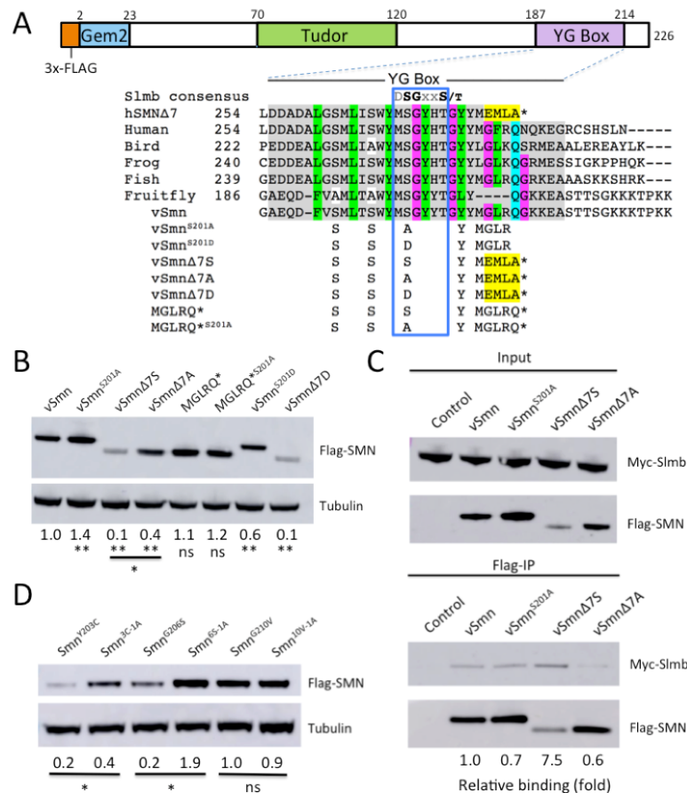
Figure 4: Identification and mutation of a putative Slmb/B-TrCP phospho-degron A . Identification of a conserved putative Slmb phospho-degron (DSGXXpS/T motif variant) in the C-terminal self-oligomerization domain (YG Box) of SMN. The amino acid sequence of Smn from a variety of vertebrates is shown to illustrate conservation of this motif and rationale for the amino acid changes. Full-length human SMN is labeled as "Human" and the truncated isoform is labeled "hSMNΔ7". Endogenous Drosophila melanogaster Smn is labeled "Fruitfly". To generate a more vertebrate-like SMN, key amino acids in Drosophila SMN were changed to amino acids conserved in vertebrates. Using this SMN backbone, a serine to alanine mutation was made in the putative degron in both full-length (vSnn S201A ) and truncated SMNΔ7 (vSnnΔ7A). An additional SMN construct that is the same length as SMNΔ7, but has the amino acid sequence GLRQ (the next amino acids in the sequence) rather than EMLA (the amino acids introduced by mis-splicing of SMN2 ) was made. The same serine to alanine mutation was made in this construct as well (MGLRQ* and MGLRQ S201A ). Finally, to mimic a phosphorylated serine the full-length SMN construct (vSnn S201D ) and truncated SMN (vSnnΔ7D) were made. B . Western blotting was used to determine protein levels of each of these SMN constructs, with expression driven by the endogenous promoter, in Drosophila S2 cells. Both the vSnn and vSnnΔ7S proteins show increased levels when the serine is mutated to an alanine, indicating disruption of the normal degradation of SMN. Additionally, MGLRQ* protein is present at higher levels than is vSnnΔ7S and protein levels do not change when the serine is mutated to an alanine. Normalized fold change as compared to vSnn levels is indicated at the bottom. *p<0.05, **p<0.01 n=3. C . Flag-tagged SMN constructs were co-transfected with Myc-Slmb in Drosophila S2 cells. Protein lysates were Flag-immunoprecipitated and probed with anti-Myc antibody to detect SMN-Slmb interaction. In both full-length SMN (vSnn) and truncated SMN (vSnnΔ7), serine to alanine mutation decreased interaction of Slmb with SMN. Truncated SMN (vSnnΔ7) showed a dramatically increased interaction with Slmb as compared to full-length SMN (vSnn), despite the fact it is present at lower levels. D . Full-length SMN constructs containing point mutations known to decrease self-oligomerization (Snn Y203C and Snn G206S ) and a mutation that does not disrupt self-oligomerization in the fly (Snn G210V ) with and without the serine to alanine mutation were transfected in Drosophila S2 cells. The constructs containing the serine to alanine mutation are as follows: Snn Y203C →Snn Y203C-1A , Snn G206S →Snn G206S-1A , Snn G210V →Snn G210V-1A . The serine to alanine mutation has a stabilizing effect on SMN mutants with poor self-oligomerization capability. *p<0.05, n=3.
