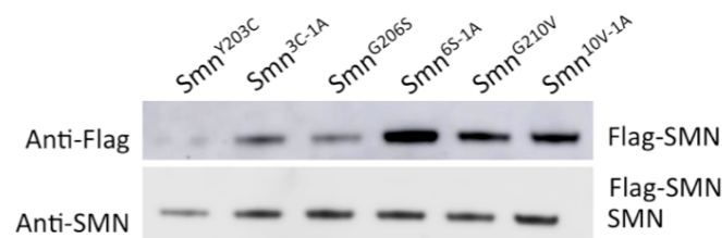
Figure S2: A) The expression of endogenous SMN in S2 cells following transient transfection of either modified 'vertebrate' SMN constructs (vSMN and vSMN S201A ) or Drosophila SMN constructs (Smn G210V and Smn 10V-1A ) is unaffected, as compared to mock transfection. Protein is detected by anti-Flag antibody or anti-SMN antibody as indicated to the left of the blots. B) Transient transfections in S2 cells express Flag-SMN from the endogenous promoter. Protein levels of all transfected constructs are lower than endogenous SMN protein levels. Protein is detected by anti-Flag antibody or anti-SMN antibody as indicated to the left of the blots.
