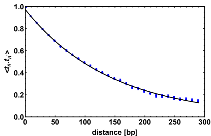
Fig. 3 The tangent-tangent correlator \langle \mathbf{t}(n) \cdot \mathbf{t}(n') \rangle computed for a chain 300 bp long; it shows an exponential decay as in Eq. (2) with a decorrelation length l_p = 143 \pm 7 bp. Points show correlations measured from the simulations (average over time), and the line shows a fit to Eq. 2. Error bars give the standard error in the mean.
