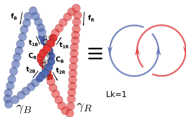
Fig. 12 The “closure” procedure can be performed on a pair of linear open curves to construct a closed pair whose linking number can be formally defined through the Gauss’ integral (see eq. (17)). In this case the curves are linked once. See text for further details.
