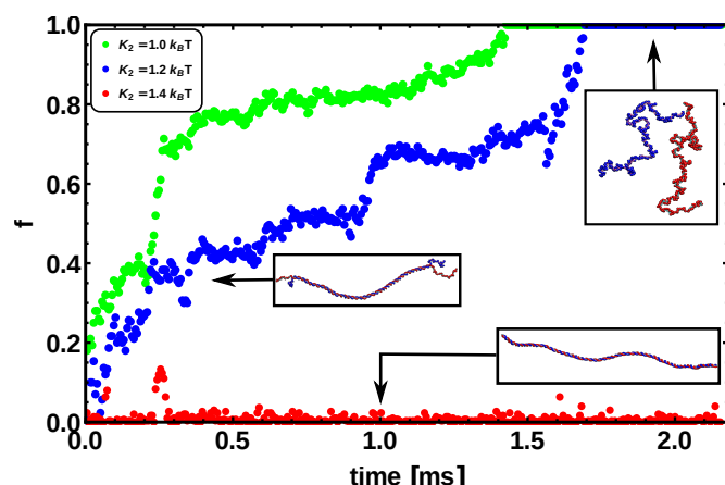
Fig. 9 This figure shows the fraction of denatured base pairs f as a function of time and for different bond energies connecting the patches of paired bases. Snapshots from simulations are also shown. The energies used range between K_2 = 1.0 k_B T and K_2 = 1.4 k_B T . We always observe that in linear dsDNA the denaturation process nucleates from the ends, as argued from experiments 65 .
