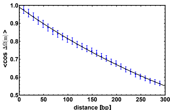
Fig. 4 The average of the cosine of the total twist angle \Delta\Omega(m) is computed for a chain 300 bp long; in this figure we show the correlator to decay exponentially as in Eq. (4) with a characteristic length l_\tau = 512 \pm 18 bp. Data points are obtained from simulations while the line is an exponential fit with f(d) = e^{-d/l_\tau} .
