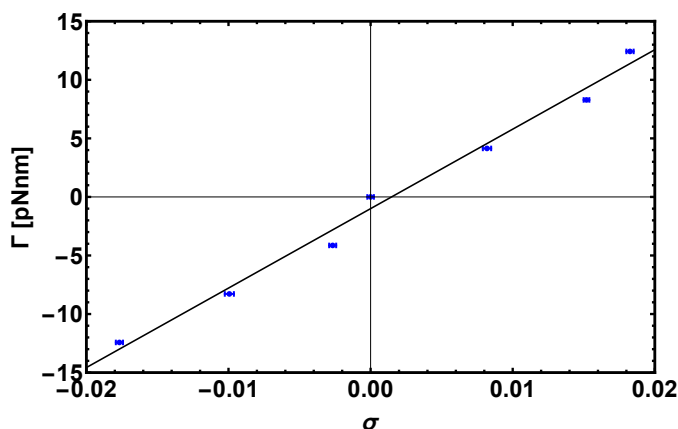
Fig. 8 Response to torque experiment. Here we show the linear regime for small |\sigma| . Fitting the data points gives the torsional rigidity C using Eq. (7).
