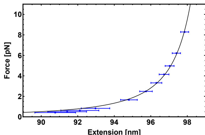
Fig. 6 Force-extension curve from the simulation (data points) and fitted by the function in Eq. (5) (solid line). The free parameters for the fitting are the total polymer length L and the persistence length l_p , both of which are in agreement with the fixed parameters of the model (see text).
