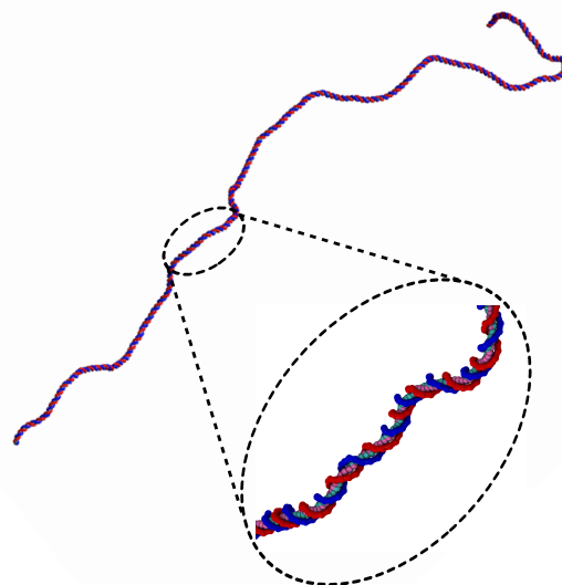
Fig. 2 An example of an equilibrated configuration of a 1000 bp double-stranded DNA molecule, as simulated with the model presented in Sec. 1.
