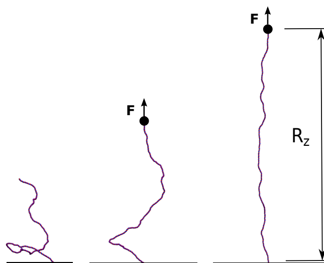
Fig. 5 In order to simulate single-molecule experiments the model for dsDNA is anchored to a surface at the bottom end while being stretched with a constant force \mathbf{F} from the top end. We then monitor the end-to-end elongation along the z -direction, R_z , and report its equilibrium value for a given force in Fig. 6.
