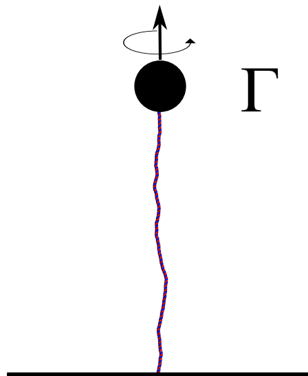
Fig. 7 The model DNA is anchored to a surface at the bottom end while being stretched with a constant force \mathbf{F} , and a torque \mathbf{\Gamma} is applied at the top end. We then monitor the linking number and report its equilibrium value for a given torque. With this information is possible to compute the superhelical density.
