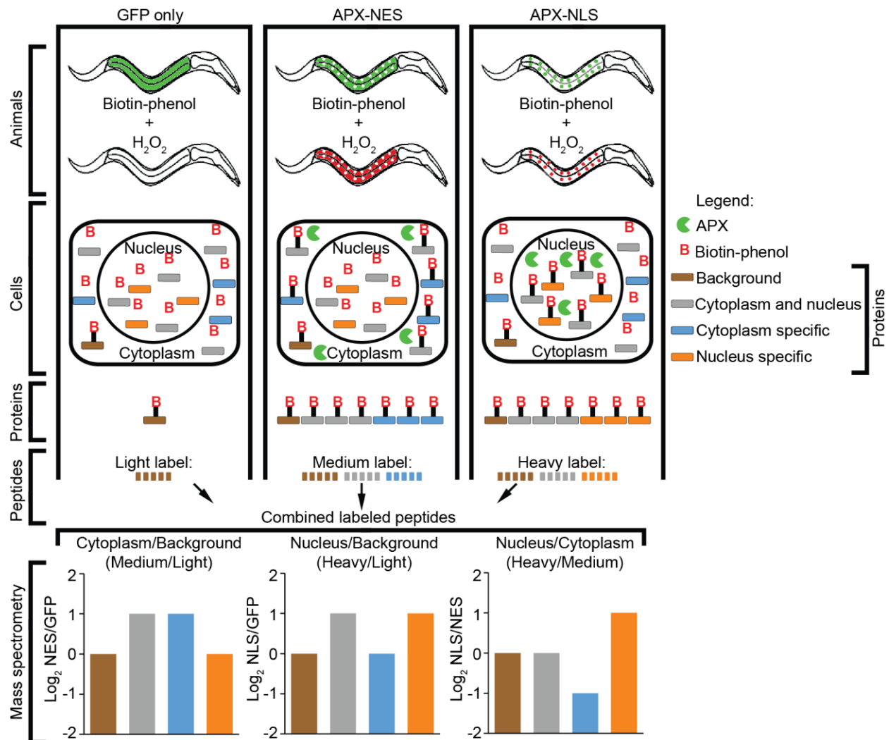
Figure 1. Overview of approach to identify tissue and subcellular-specific protein expression in C. elegans . Schematic of spatially restricted enzymatic tagging in C. elegans . Animal strains are generated that express the APX enzyme in either the cytoplasm or the nucleus in a tissue-specific manner, such as in the intestine as illustrated here. Animals are treated with biotin-phenol that diffuses into cells. The APX enzyme, in presence of H_2O_2 and biotin-phenol catalyzes the formation of a phenoxyl radical that covalently labels neighboring proteins with biotin (red B with black bars) 13 . Thus, biotin labeling (labeled in red) of proteins occurs in whichever specific tissues and subcellular locations the enzyme is expressed. Three strains are used to measure protein localization in each tissue: GFP only, GFP-APX-NES, and GFP-APX-NLS. Spatially restricted tagging is performed using these three strains and then the proteins are extracted and purified using streptavidin beads. These purified proteins are then digested into peptides and labeled using reductive dimethyl labeling for quantitative comparisons between the three strains. The peptides from each sample are then combined and peptide ratios in each sample are measured using mass spectrometry. The peptide ratios can then be used to determine if the protein is detected over background and if it is enriched in either the nucleus or cytoplasm.
