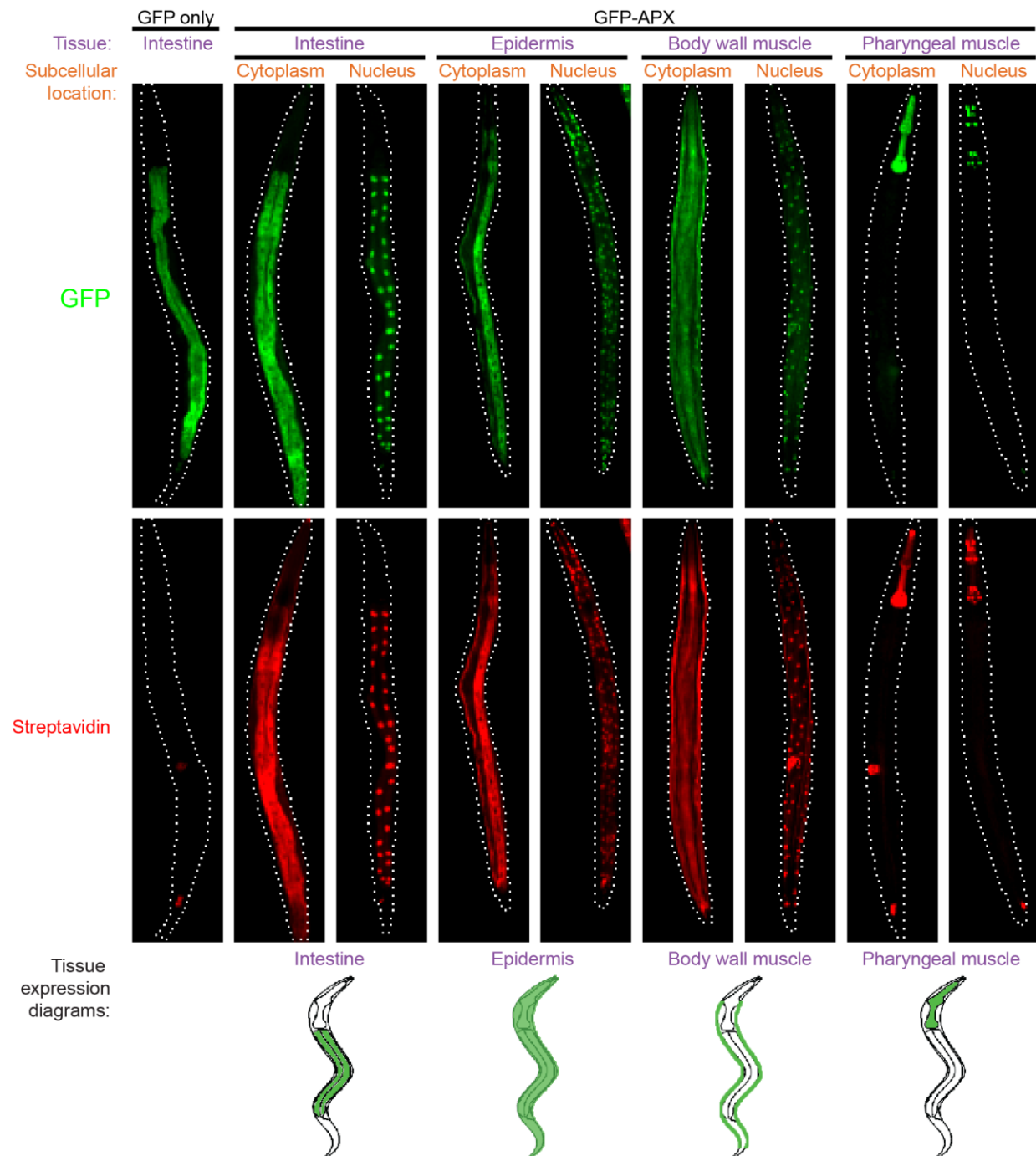
Figure 3. APX-mediated biotin labeling in vivo displays tissue and subcellular specificity.
