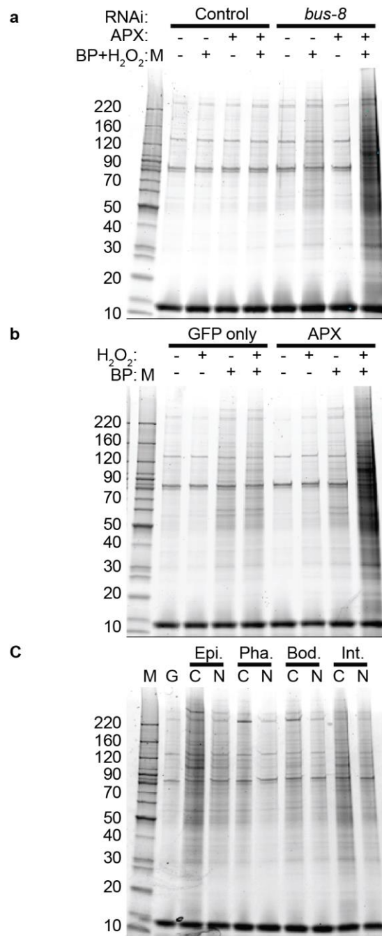
Figure 2. Efficient spatially restricted enzymatic tagging in C. elegans is dependent on biotin-phenol, H 2 O 2 , and bus-8 RNAi. a-c. Streptavidin-purified proteins from C. elegans protein extracts were visualized with the Oriole stain. a. Animals expressing GFP-APX (APX +) in the intestinal cytoplasm or a GFP only control strain (APX -) were grown on plates with either control (L4440) or bus-8 RNAi. Animals were either treated or untreated with biotin-phenol (BP) and H 2 O 2 . Protein markers are indicated (labeled M). b. Animals expressing GFP-APX in the intestinal cytoplasm or a GFP control strain grown on plates with bus-8 RNAi were treated with either H 2 O 2 or biotin-phenol, or both. c. Strains of C. elegans expressing GFP-APX in either the cytoplasm
