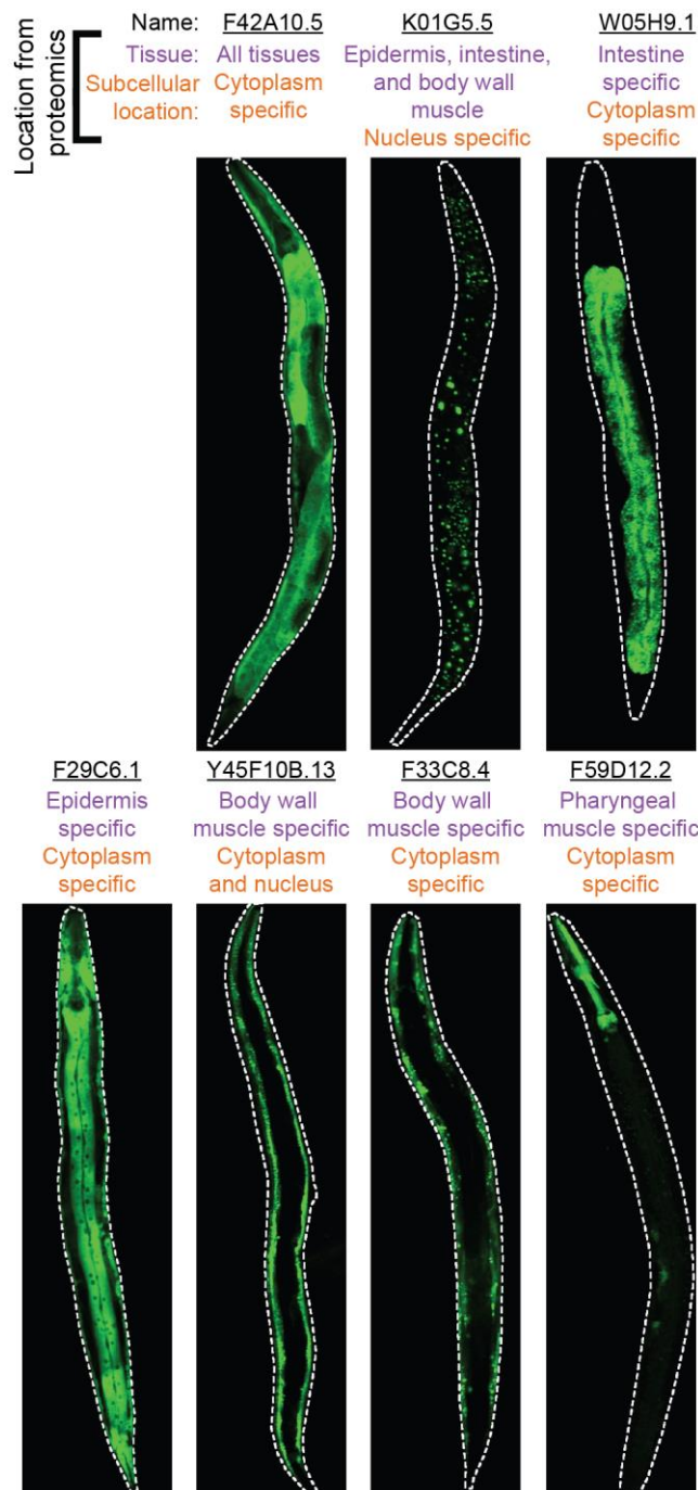
Figure 5. Validation of identified protein locations using fluorescently-tagged proteins.
