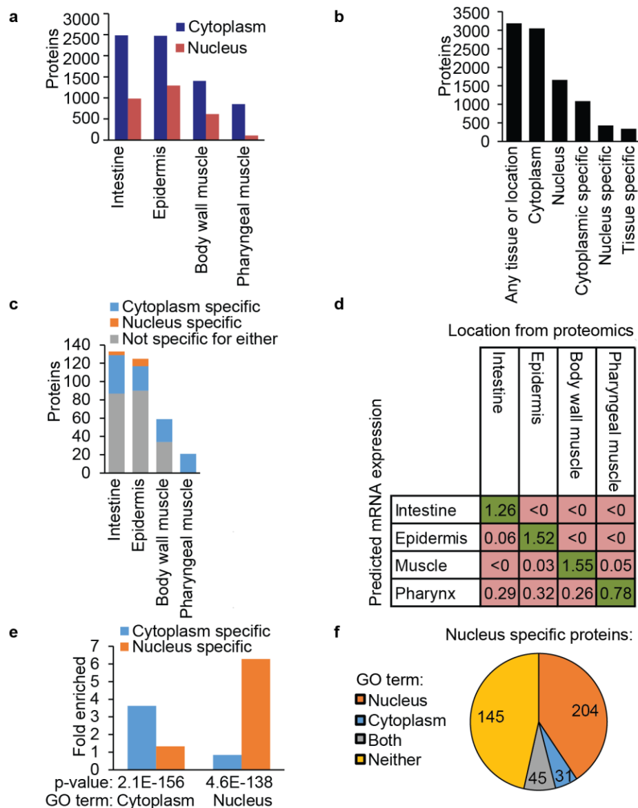
Figure 4. Identification of C. elegans proteins with tissue- and subcellular-specific localizations. a. The number of proteins identified above background from the tissue or subcellular location for each of the eight locations indicated. b. The total number of proteins identified in our experiments that were detected in different locations or that were detected as being specific to a location. c. The number of proteins we identified in the indicated tissue, but not in the other three tissues. For each tissue, three categories of proteins are shown, those that are specific to the cytoplasm (orange), those that are specific to the nucleus (blue), and those that are not specific to either compartment (grey). d. Comparison of the identified tissue-specific proteins to a dataset of predicted mRNA expression 20 . The data presented are the average of all the mRNA expression prediction scores for each tissue-specific protein in each of the four tissues. Higher prediction scores are more likely to be expressed in that tissue. Each column represents proteins identified as specific to that tissue, compared to the predicted mRNA expression of the tissue in each row. The highest average score in each column is shaded in green, and all other
