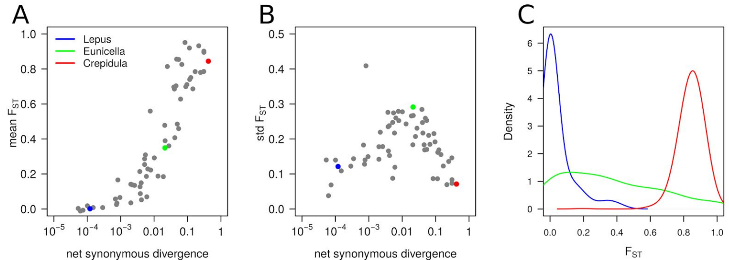
Figure S3. Relation between synonymous divergence and genetic differentiation.
