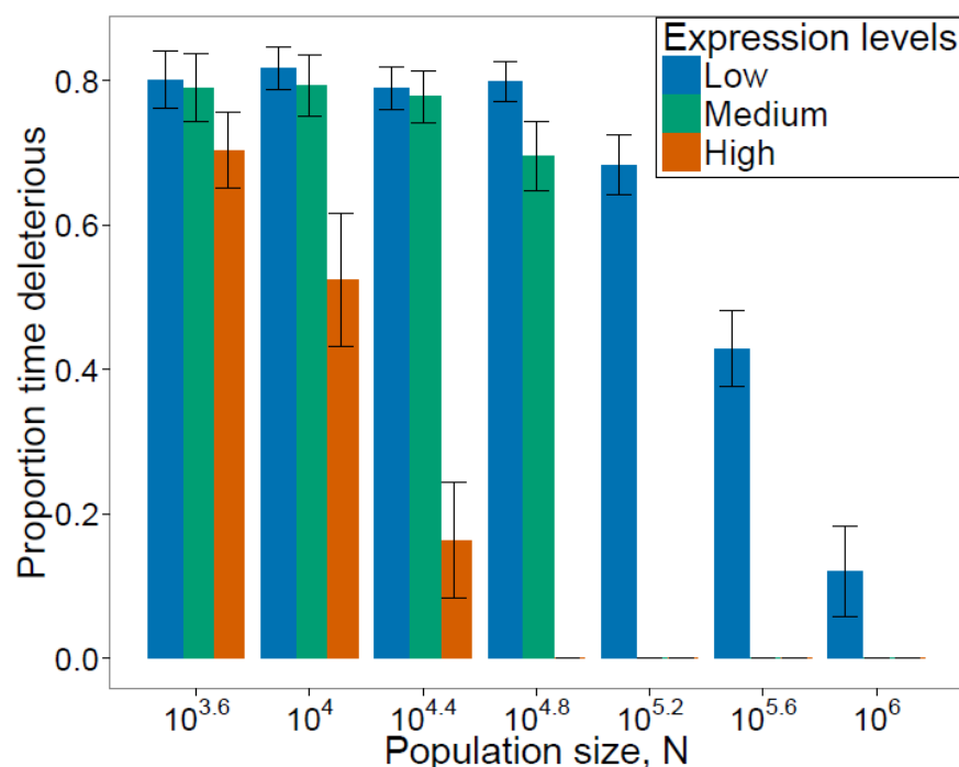
Figure 2: The effectiveness of purging a cryptic sequence of deleterious mutations depends on its expression level. We examined the states of the cryptic sequences of the loci with the 10 highest, the 10 lowest, and the 10 median expression levels among the 600 loci in each of the simulations showed in Fig. 1 ( \sigma_E = 2.25 ). We counted how often each locus contained a deleterious cryptic sequence among the last 20 timepoints we had collected from that simulation. Bars represent the proportion of time that each of the 10 loci carried a deleterious cryptic sequence, averaged over 20 replicates, and shown as \text{mean} \pm \text{SD} . Simulations were initialized at low- p conditions.
