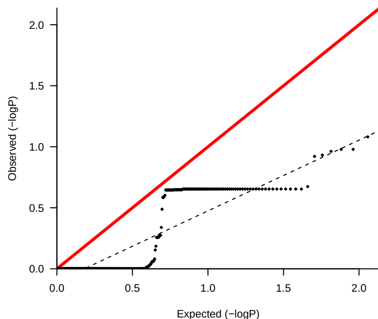
lambda 0.58
