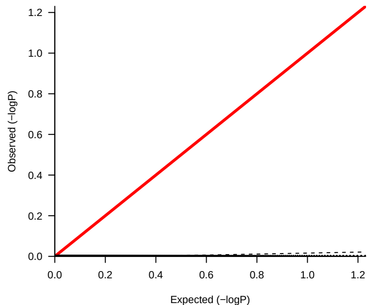
lambda 0.024
