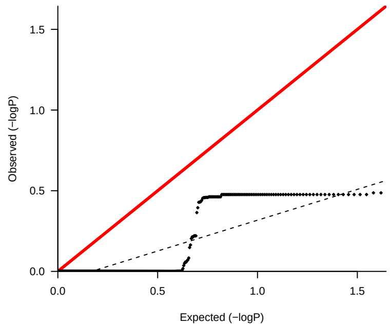
lambda 0.382
