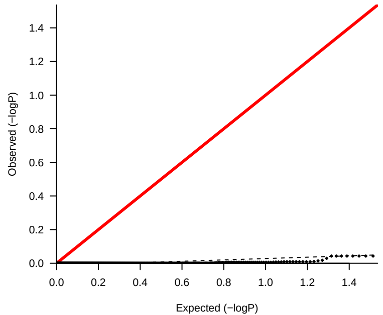
lambda 0.04
