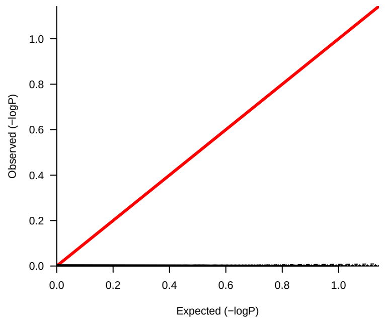
lambda 0.012
