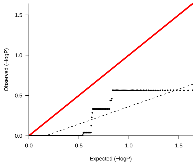
lambda 0.434
