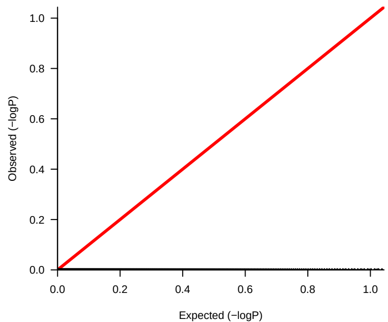
lambda 0.004
