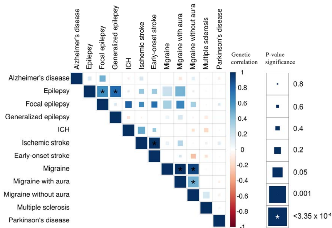
Figure 2. Genetic correlation matrix across neurological phenotypes.
