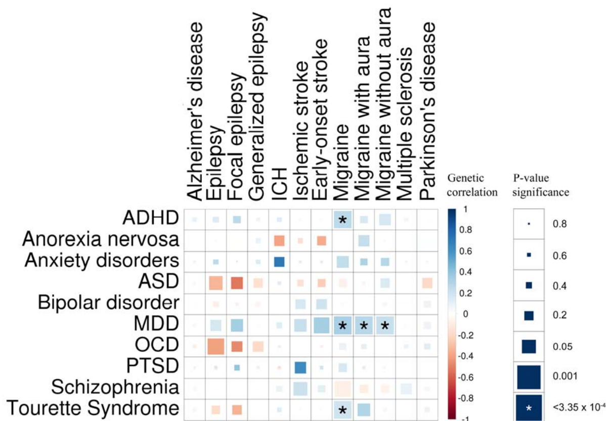
Figure 3. Genetic correlation matrix across neurological and psychiatric phenotypes.
