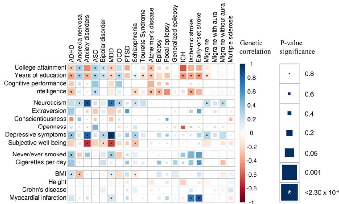
Figure 4. Genetic correlation matrix across brain disorders and behavioral-cognitive phenotypes.
