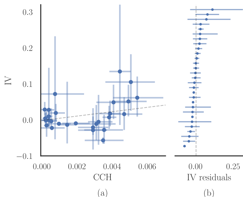
Figure 6: IV and CCH estimates on hippocampal recordings. IV and CCH estimates for connections from optogenetically activated to non-activated units that showed a significant peak in the CCH (English et al., 2017). (a) Blue dots are median values and error bars indicate the 95% confidence intervals calculated by bootstrapping ( n = 1000 ). Dashed line represents linear fit of median values, which we show because CCH estimates may be linear biased. For better visualization, we omitted one estimated connection at CCH = 0.01 and IV = 0.36 . (b) Sorted IV residuals and errorbars in relation to the linear fit (vertical line). In many cases, 95% confidence intervals do not overlap with linear fit.
