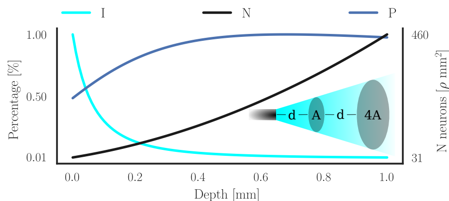
Figure 1: Spatial extent of optogenetic stimulus. Due to scattering and geometric loss the light intensity (I, cyan line) with an intensity of 10 \text{ mW/mm}^2 exiting the optogenetic fiber follows approximately an inverse square law r^{-2} where r is the distance from the fiber. If neurons are uniformly distributed, the number of affected neurons in a spherical slice increases by r^2 (N, black line). The total photo current (P, blue line) calculated as the sum over neurons of peak amplitude photo current in a spherical slice thus increases with distance due to the nonlinear relation between light intensity and photo current, depicted as percentage of maximum.
