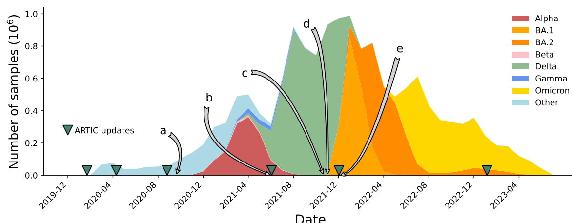
Figure 2: Timeline of the SARS-CoV-2 pandemic from December 2019 to July 2023, with selected events relating to problems with sequencing and consensus calling labelled a-e. Releases of ARTIC primers schemes (versions 1, 2, 3, 4, 4.1, 5.3.2) are marked with green triangles. a) Primer dimers cause amplicon dropouts [10] and 28% of GISAID [11] sequences deposited in September 2020 have at least one gap of length at least 200bp [12]. b) A 9bp deletion in the primer binding region of ARTIC V3 amplicon 73 causes missing data [13]. c) Dropouts causing artefacts at Spike 95 and 142 [14]. d) ARTIC v4 roll out triggers artifactual mutations in some pipelines [15]. e) Omicron samples cause ARTIC v4 amplicon dropout, triggering the update to ARTIC v4.1 [16].
