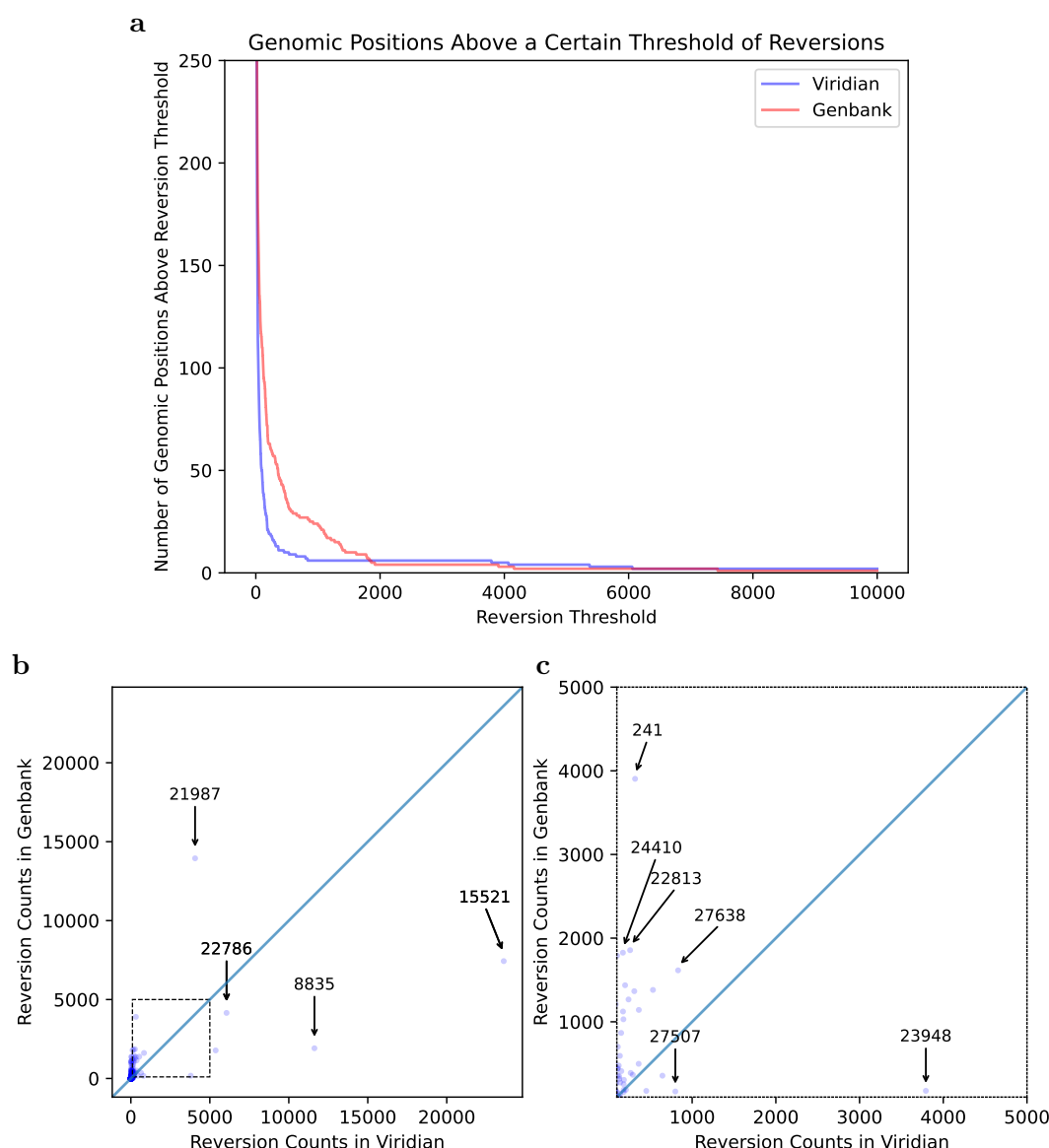
Figure 4: Most variable sites cause fewer reversions in the Viridian tree than the GenBank tree. a) Plot showing how many positions in the genome (y axis) have at least N reversions (x axis) in each tree (Viridian in blue, GenBank in red). Viridian curve drops faster, having fewer positions that create many reversions. b) Scatterplot comparing count of reversion mutations found in GenBank Dataset (y axis) and Viridian dataset (x axis). Note (0,0) is slightly indented from the origin of the plot. Each point represents a position of the SARS-CoV-2 genome. Three points below the line y=x are highlighted (labelled by genomic coordinates: 22786, 8835, 15521) where Viridian has particularly high numbers of reversions, and one (labelled 21987) for GenBank. c) Blow up of dotted square from panel b) showing vast majority of variable sites in the genome lie above the line y=x .
