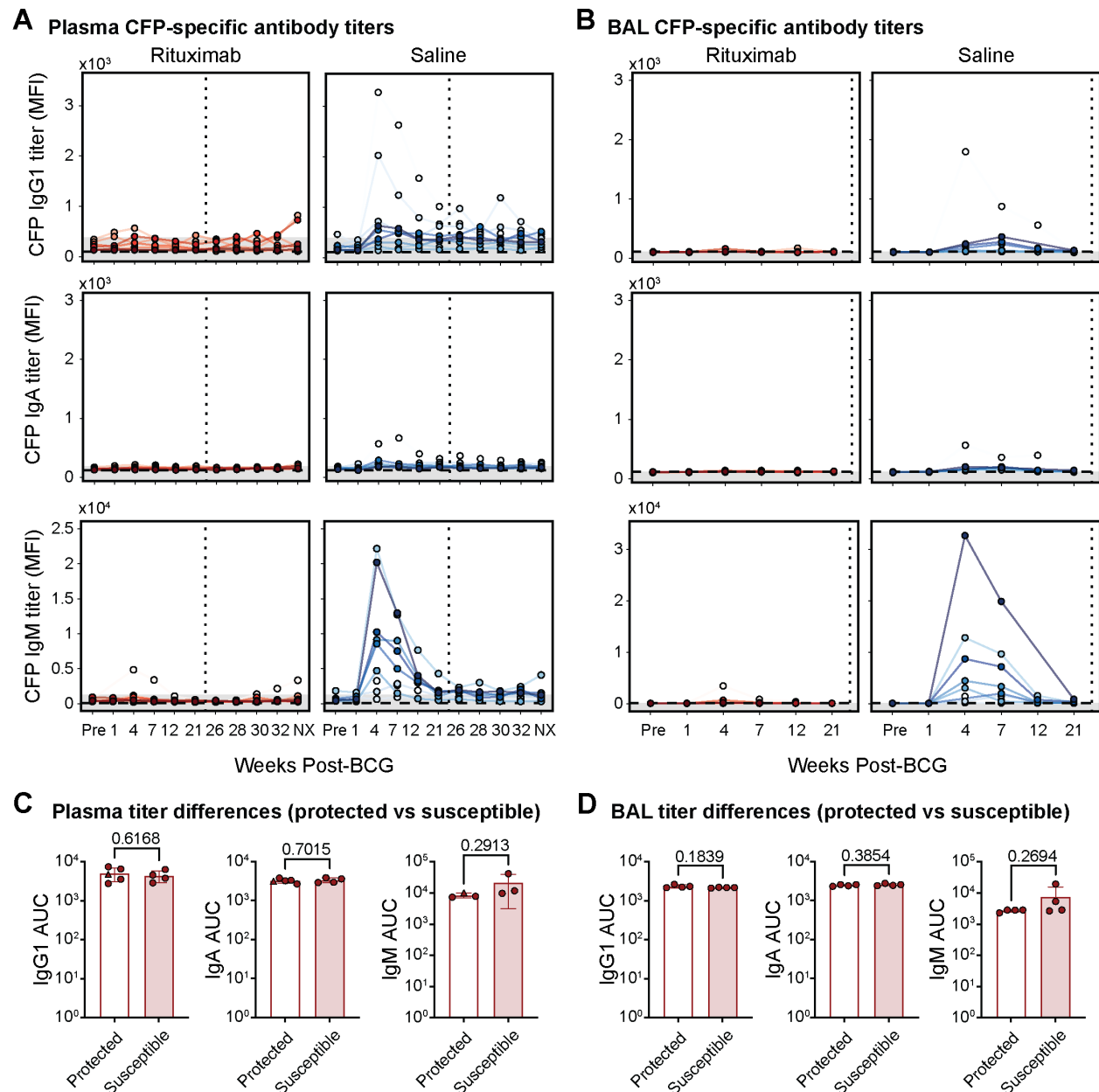
Figure S5. CFP-specific antibody responses. A, B) IgG1 (top), IgA (middle), and IgM (bottom) antibody titers present in the (A) plasma, and (B) BAL, of each macaque following IV BCG vaccination specific to CFP measured via Luminex. Y-axis is median fluorescence intensity (MFI). X-axis shows time
